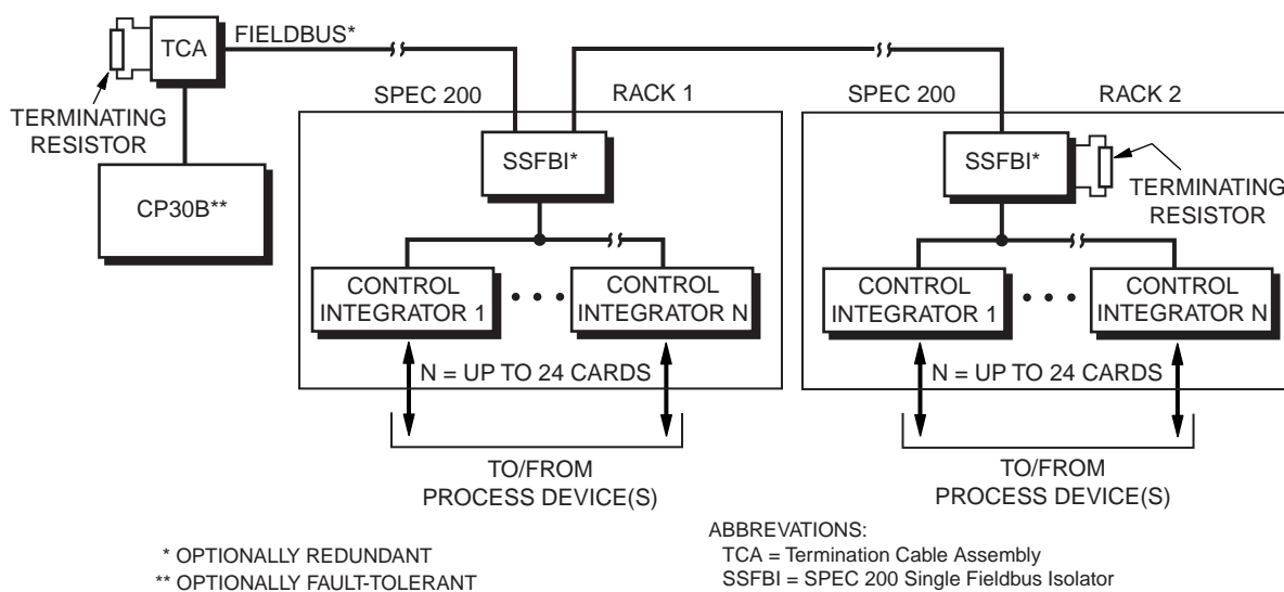
Figure 8. Twinaxial Fieldbus SPEC 200 Control Subsystem Interface Configuration (Typical Configuration)
