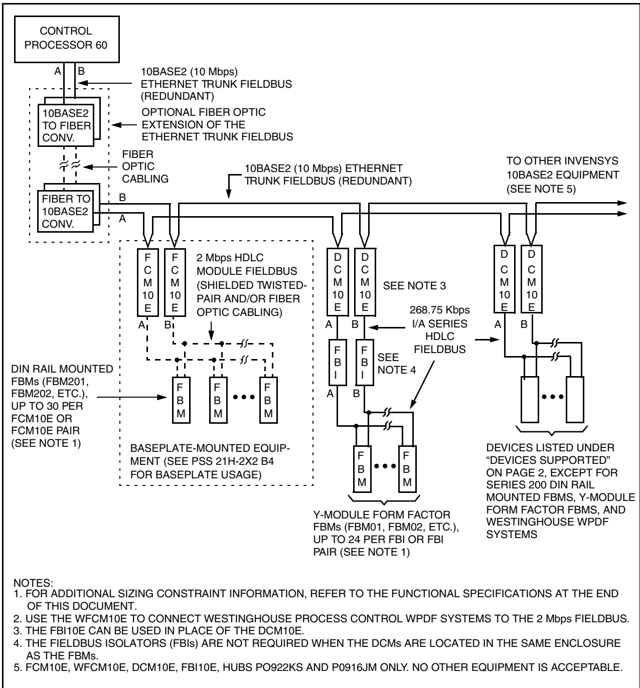
Figure 1. Typical Direct Network Configuration
