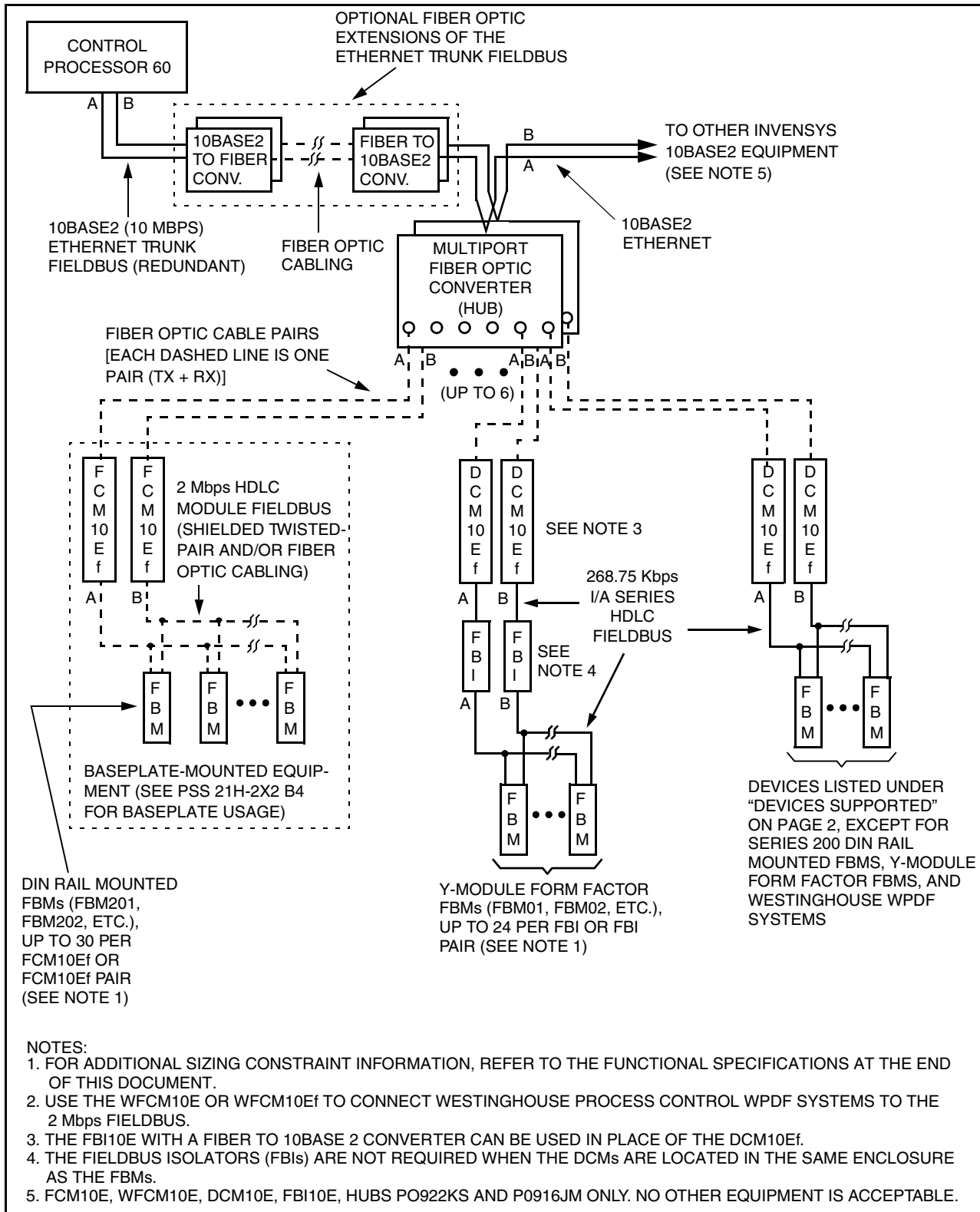
Figure 2. Typical Active Star Network Configuration
