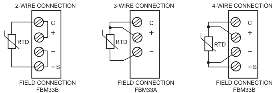
Figure 1. Input Connections
