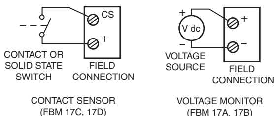
Figure 8. Digital Input Configurations (TAA17)
