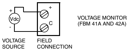
Figure 13. Input Configurations (TAA41)
