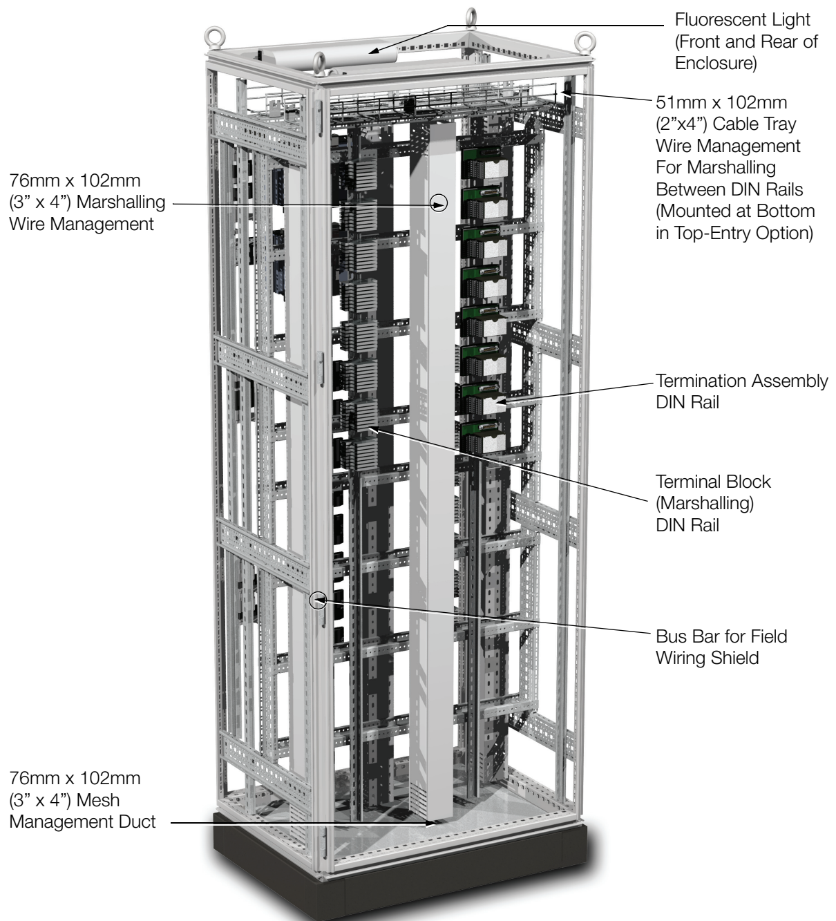
Figure 3. G21 Termination Enclosure with Marshalling Option, Rear View, Bottom Entry
