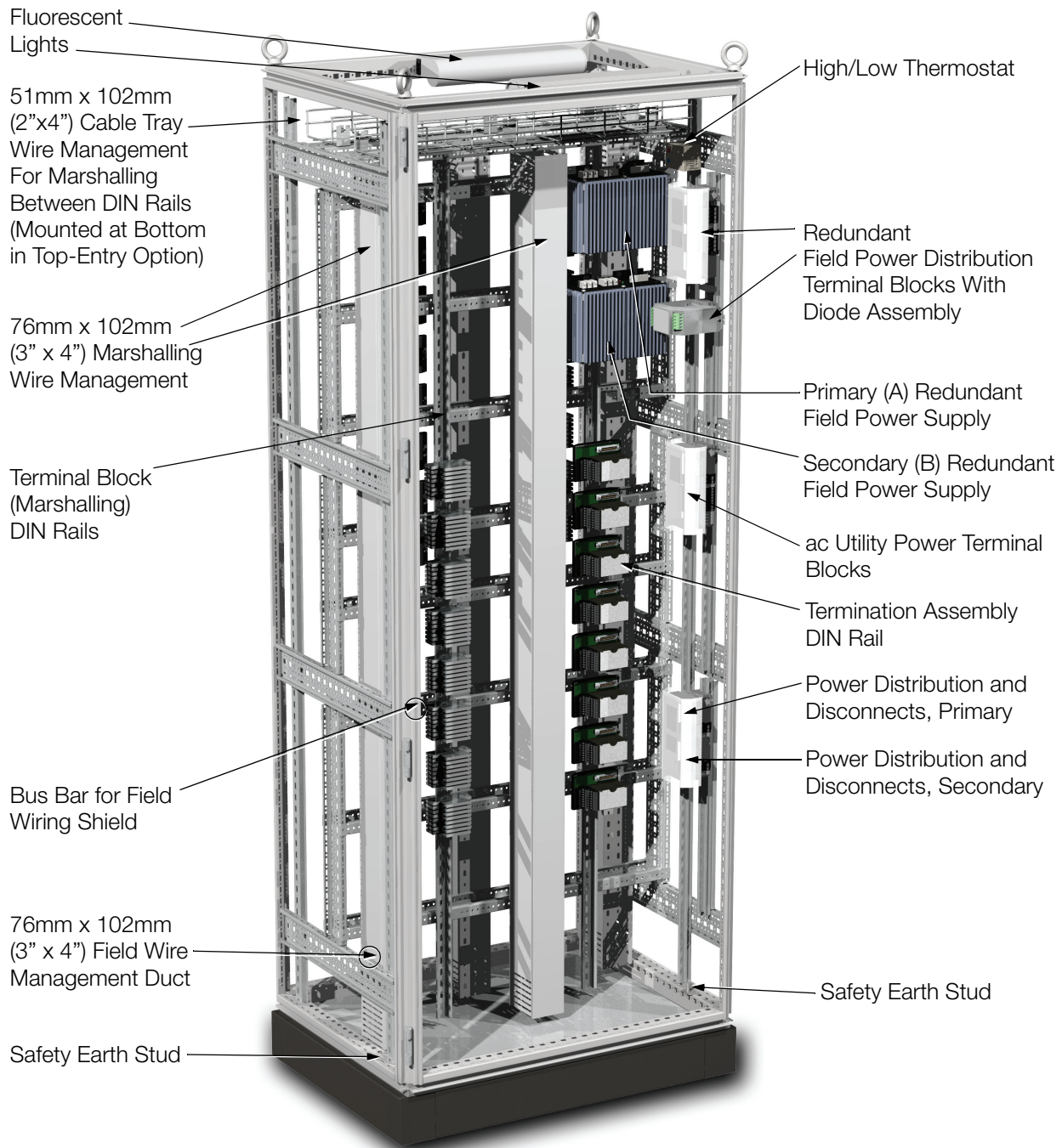
Figure 2. G21 Termination Enclosure with Marshalling Option, Front View, Bottom Entry
