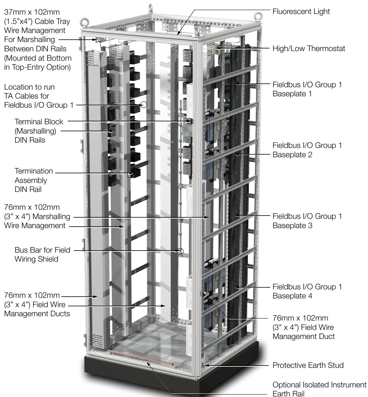
Figure 2. G17 System and Termination Enclosure, Front Right View
