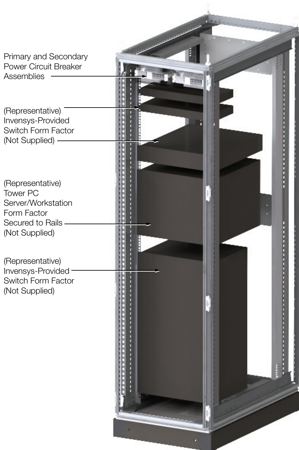
Figure 10. G50 Server Enclosure With Server, Top Entry, Rear View
