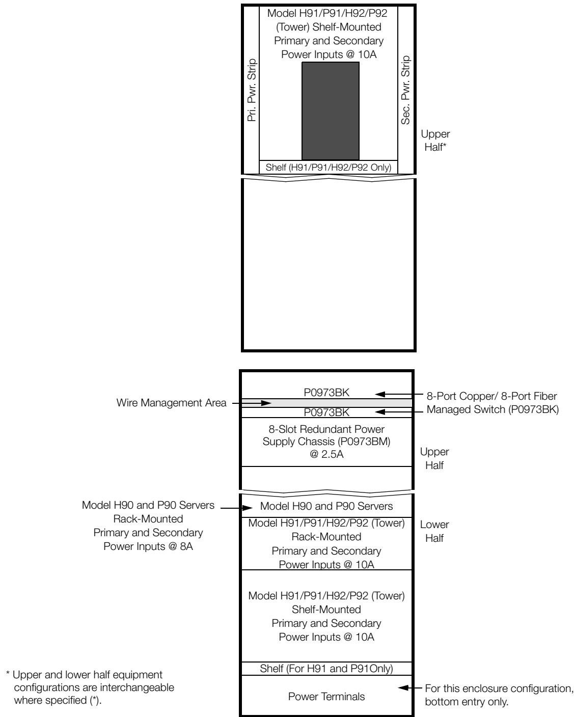
Figure 3. Example Configurations for I/A Series Workstations and Servers in G50 Enclosure (Part 2)
