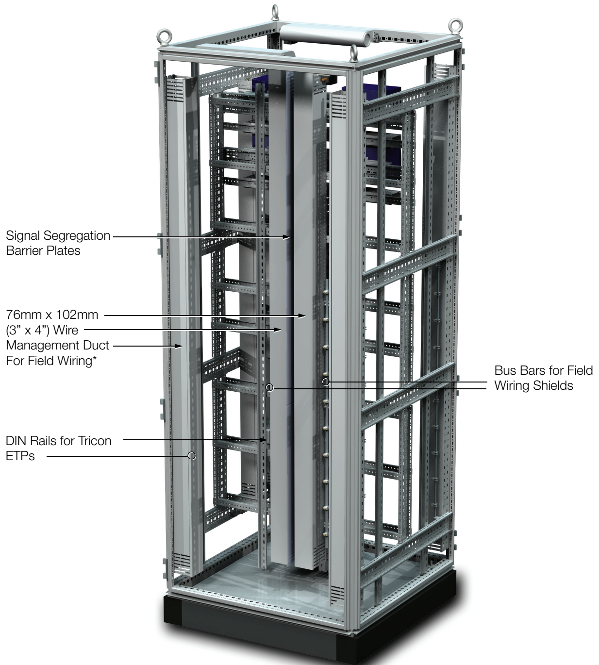
Figure 5. G61 Tricon Termination Enclosure with Termination Option, Rear View, Bottom Entry
