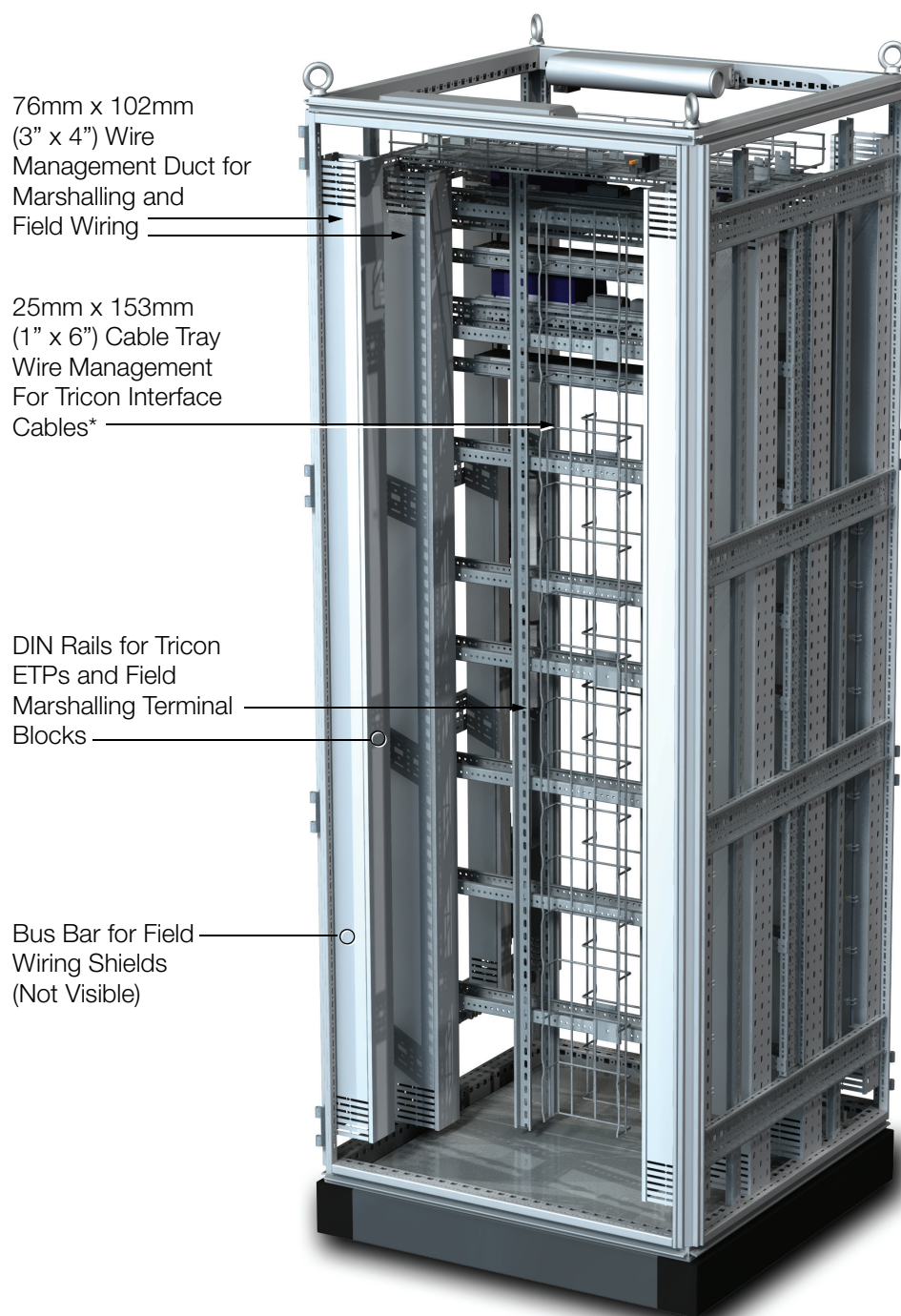
Figure 3. G61 Tricon Termination Enclosure with Marshalling Option, Rear View, Bottom Entry
