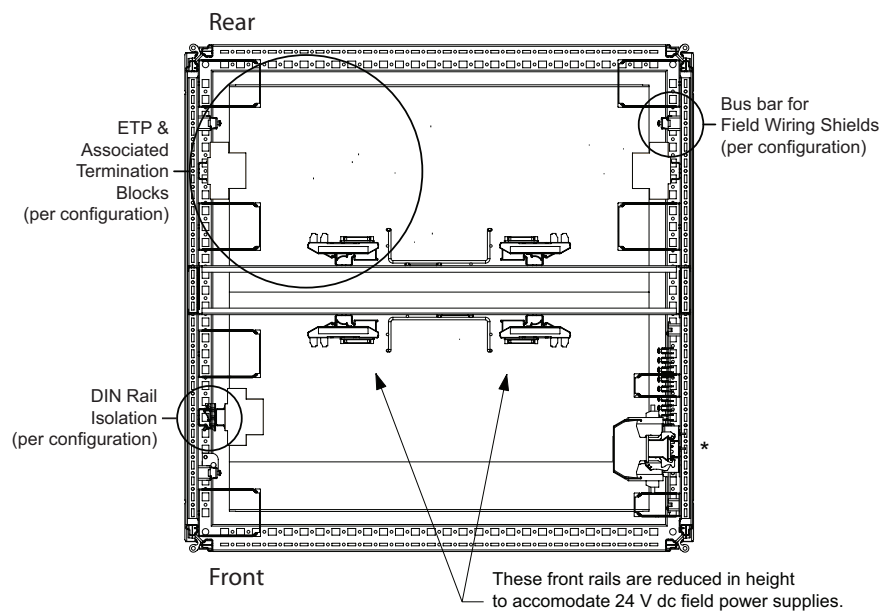
Figure 1. G61 Tricon Termination Enclosure Termination and Marshalling Layouts and DIN Rail Identification
