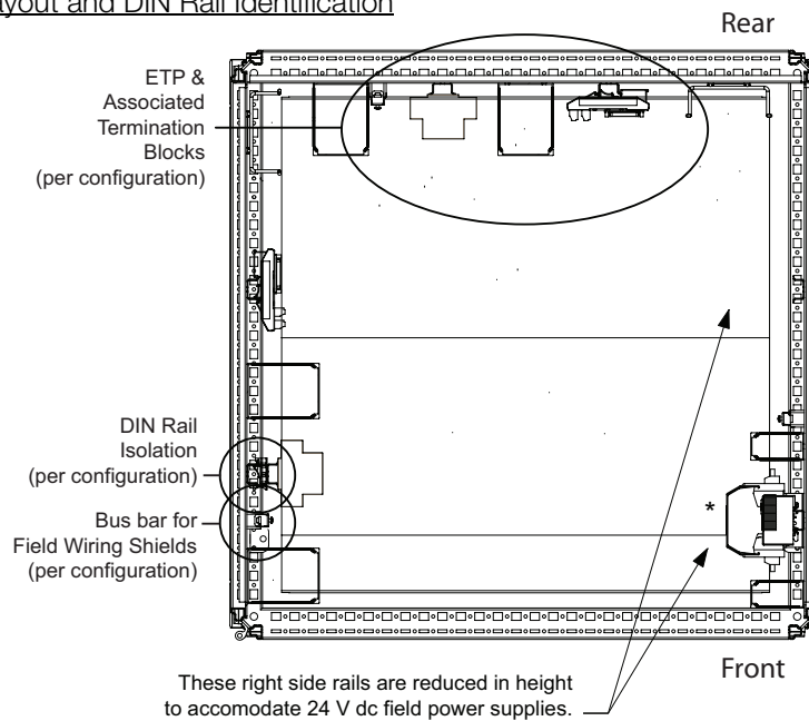
Figure 1. G66 Tricon Termination Enclosure Termination and Marshalling Layouts and DIN Rail Identification
