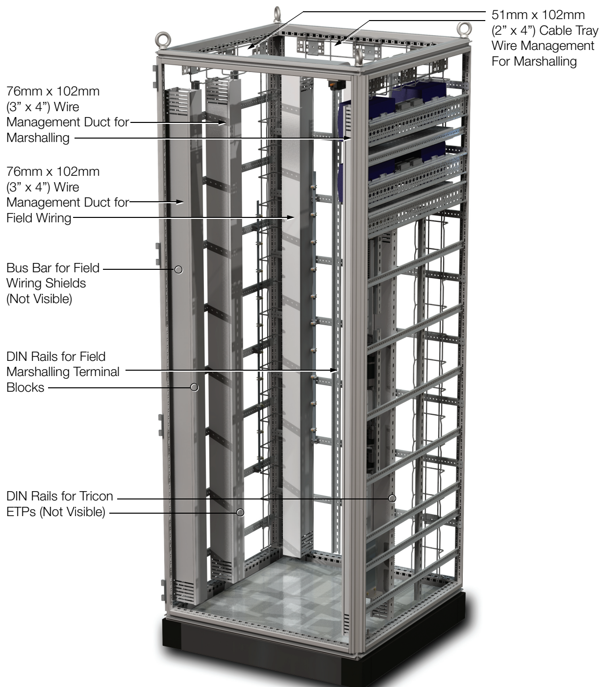
Figure 3. G66 Tricon Termination Enclosure with Marshalling Option, Front Left View, Bottom Entry
