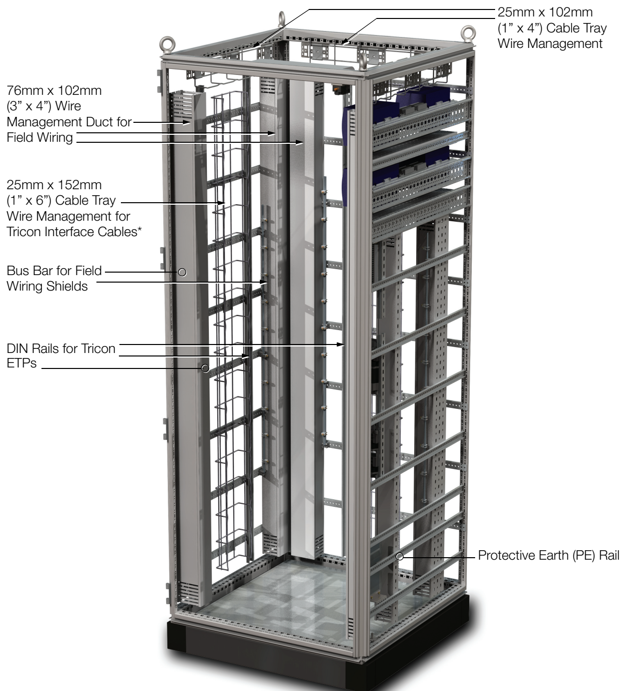
Figure 5. G66 Tricon Termination Enclosure with Termination Option, Front Left View, Bottom Entry
