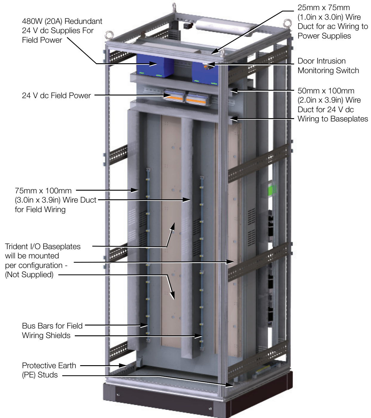
Figure 3. G80 Trident System Enclosure, Rear Right View
