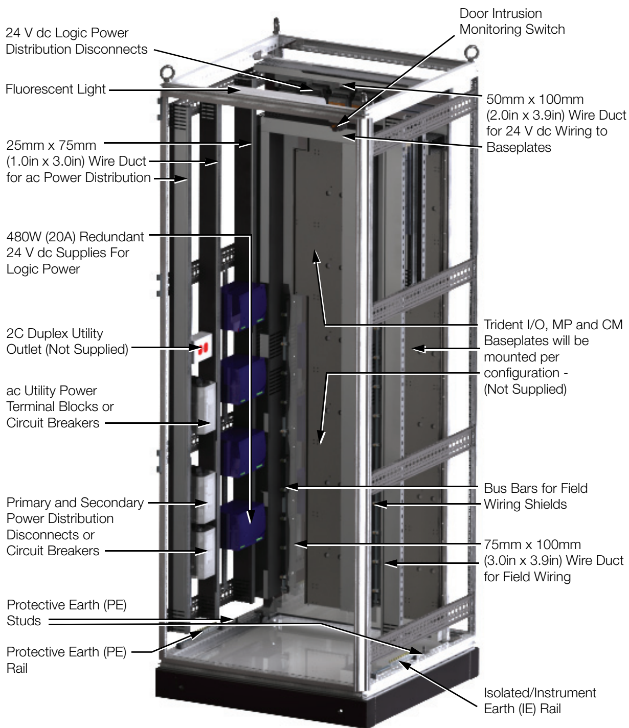
Figure 1. G85 Trident System Enclosure, Front Left View
