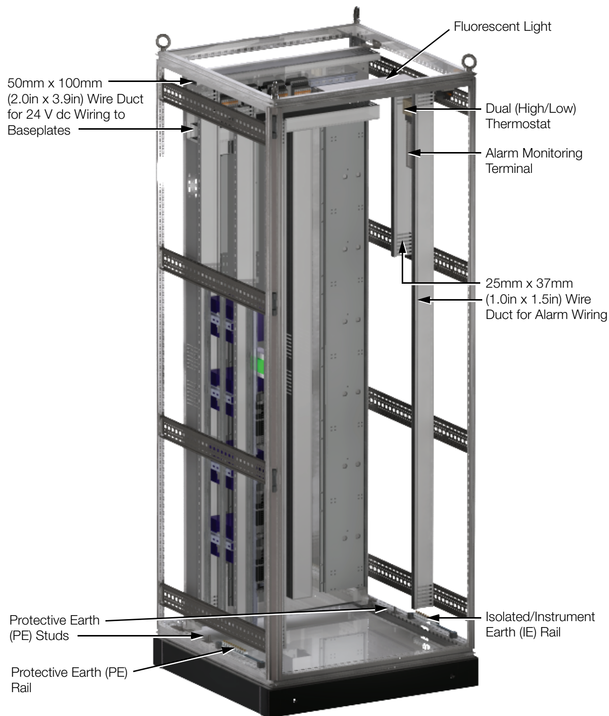
Figure 2. G85 Trident System Enclosure, Front Right View
