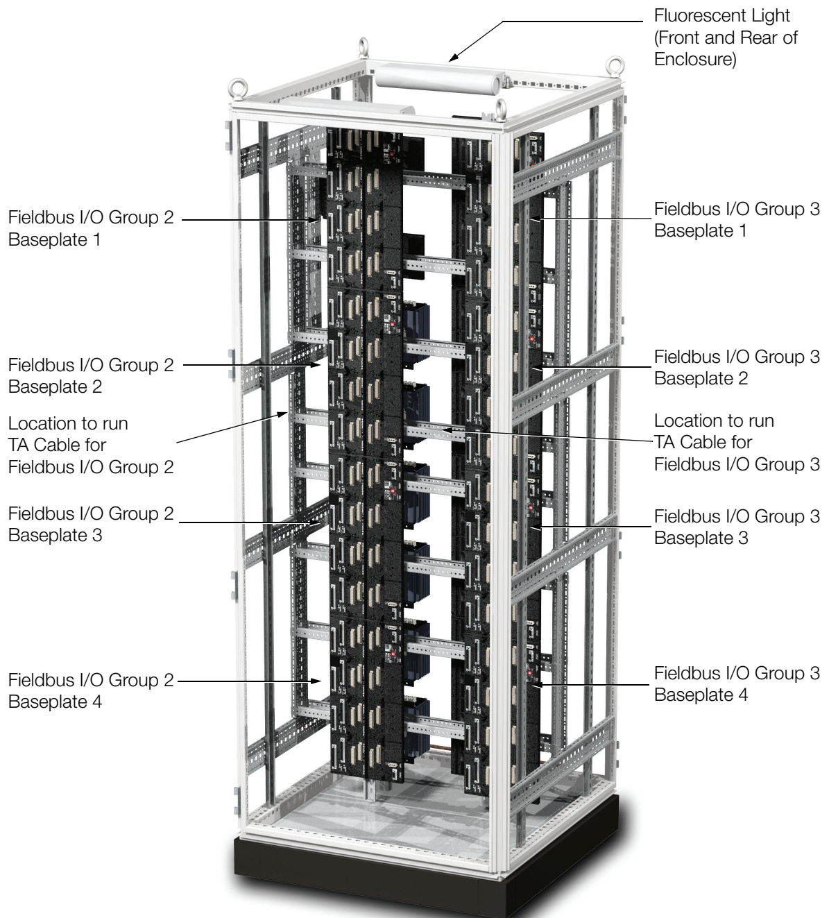
Figure 2. G10 System Enclosure, Rear View
