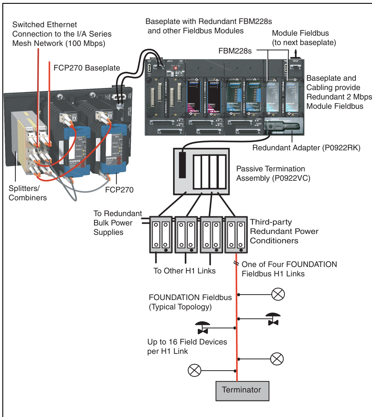
Figure 2. Generic Connection of FBM228 Power Conditioners
