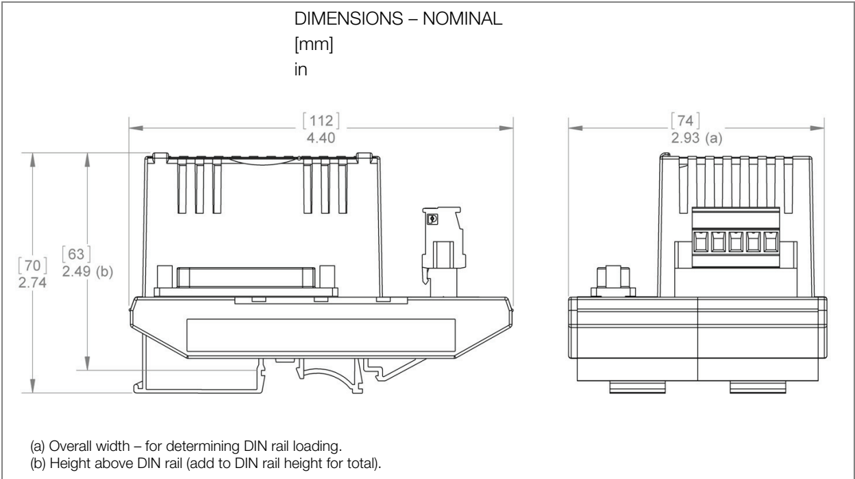
Figure 2. Termination Assembly (P0926TE)
