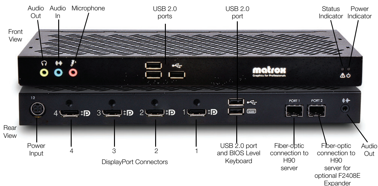
Figure 1. Remote Graphics Unit for H90 Servers (Front and Rear Views)
