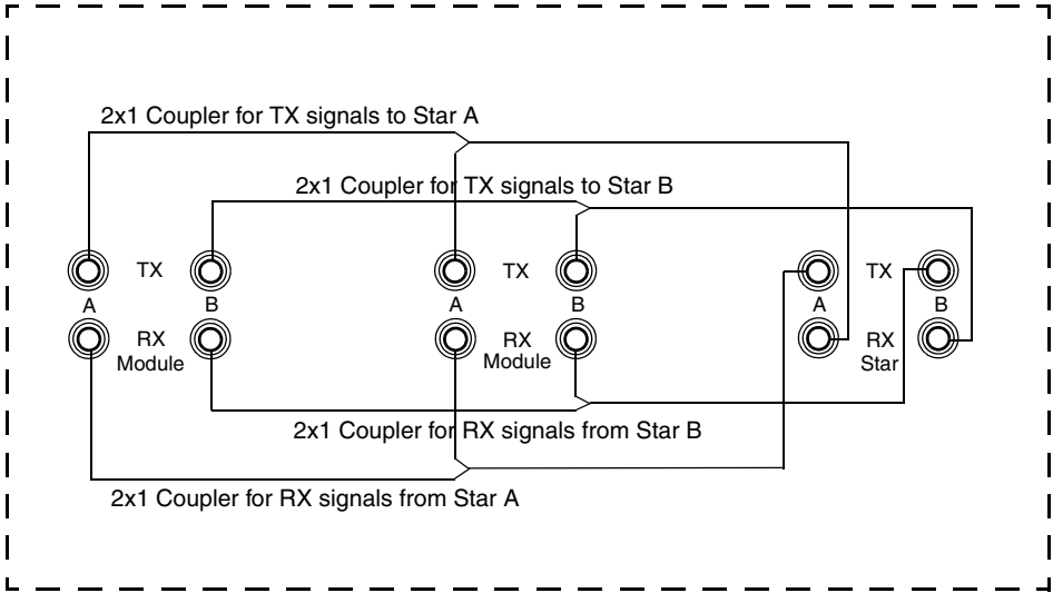
Figure 2. Splitter/Combiner (Internal)
