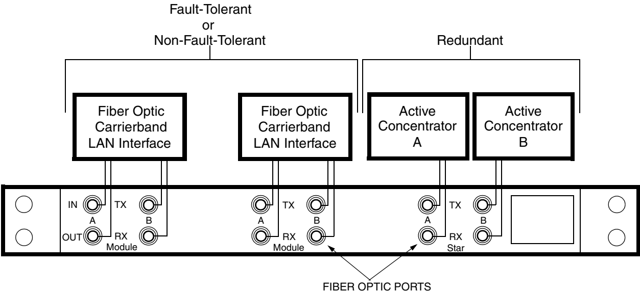
Figure 1. Splitter/Combiner Connections
