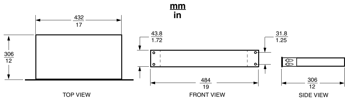
Figure 4. Splitter/Combiner Dimensions
