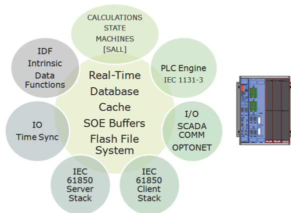
Figure 1. Real-Time Database and Environment
