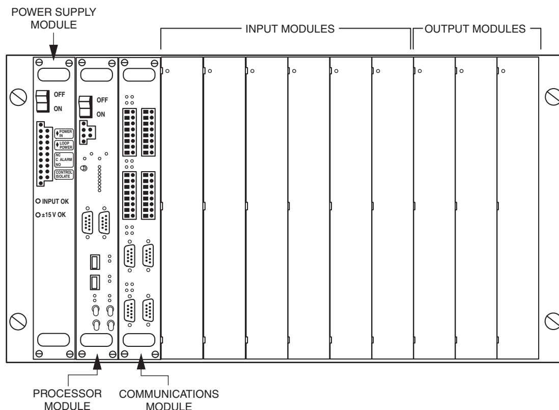
Figure 2. I/A Series SCD5200 Ten I/O File Power Supply System, Example Implementation
