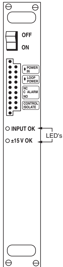
Figure 3. Front Panel
