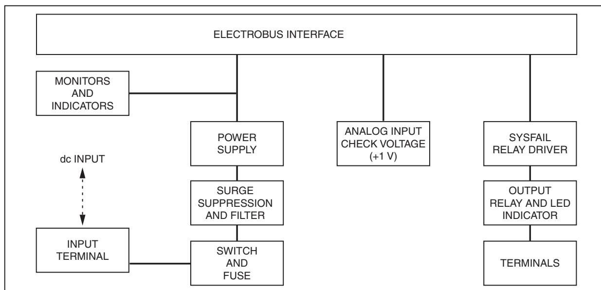
Figure 1. I/A Series SCD5200 Power Supply Module Functional Block Diagram
