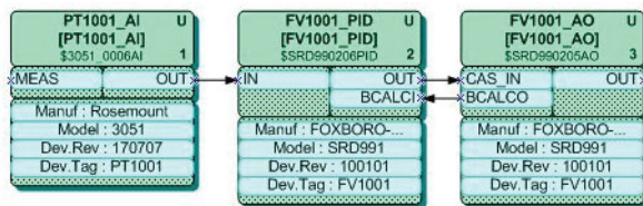
Figure 1. Block Diagram Typical CIF Loop
