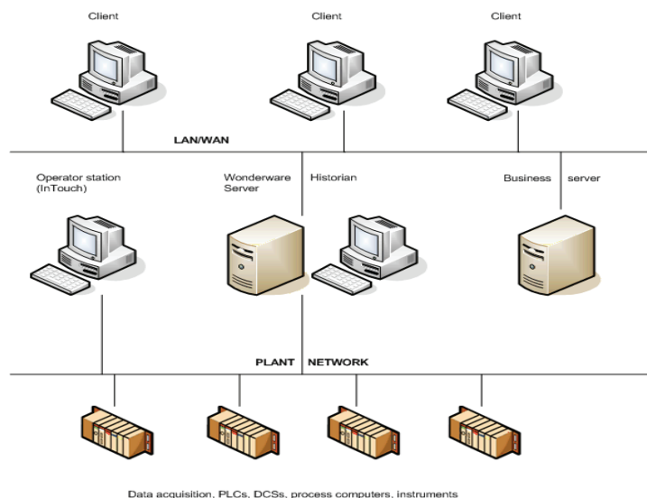
Figure 8. Process and IT Network Architecture with Wonderware Historian
