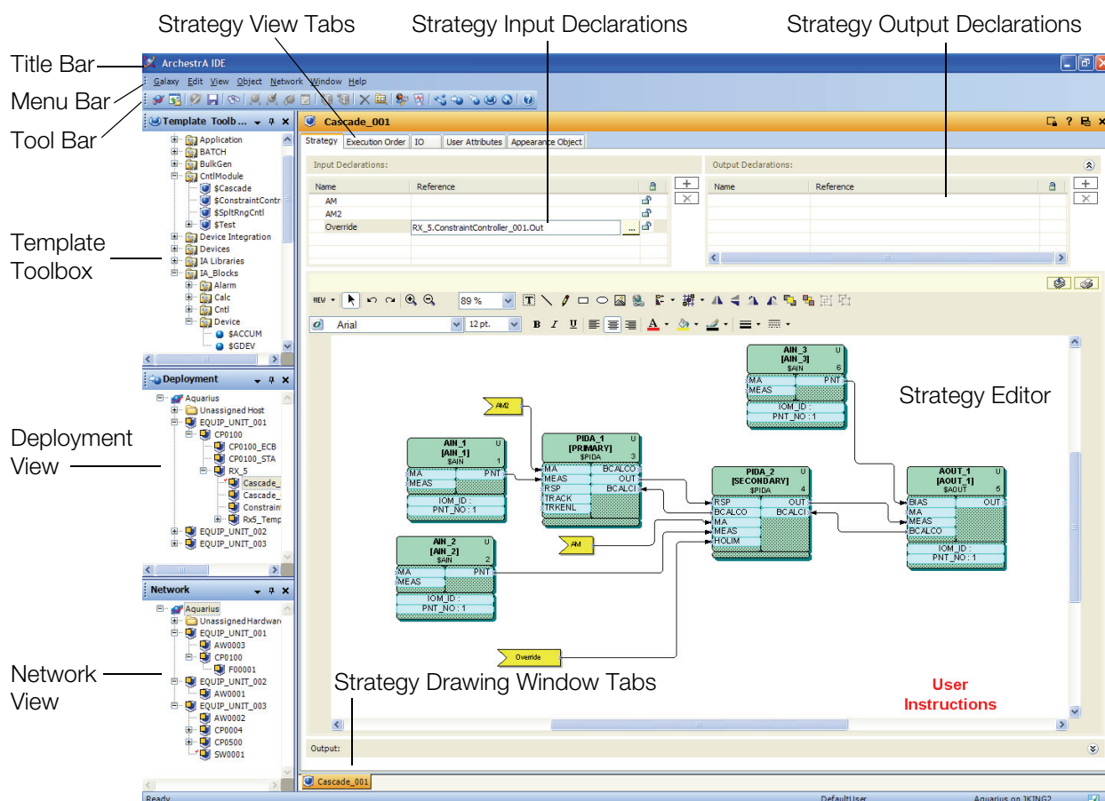
Figure 1. Foxboro Control Software Configuration Tools Navigation
