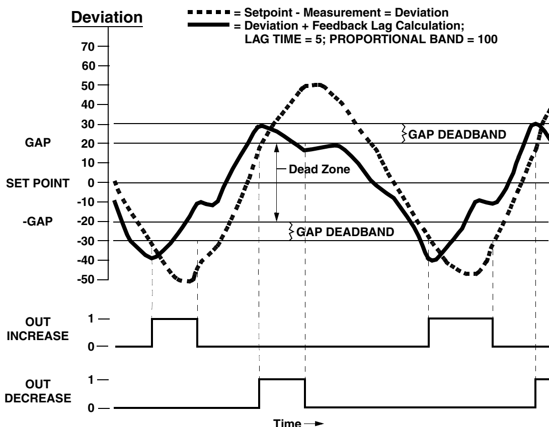
Figure 3. Feedback Lag Algorithm Timing Diagram
