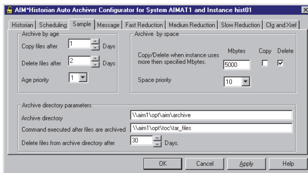
Figure 9. AutoArchiver Configurator Sample Page
