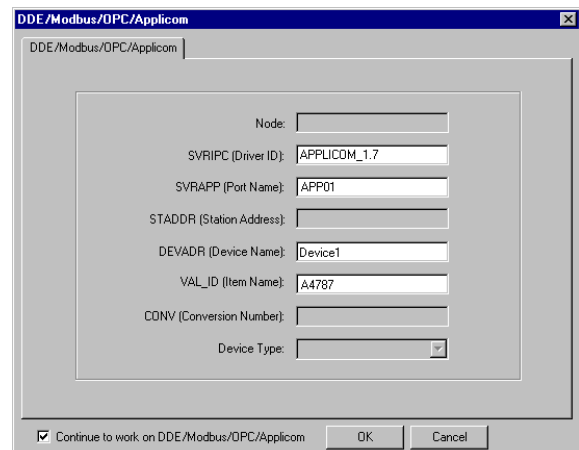
Figure 3. Applicom Dialog Box
