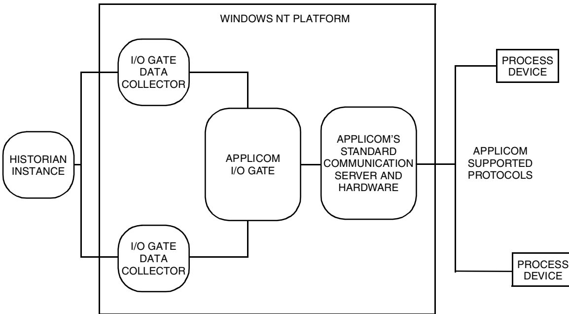
Figure 1. Open Device Integration Architecture Showing a Applicom I/O Gate with Other I/O Gates
