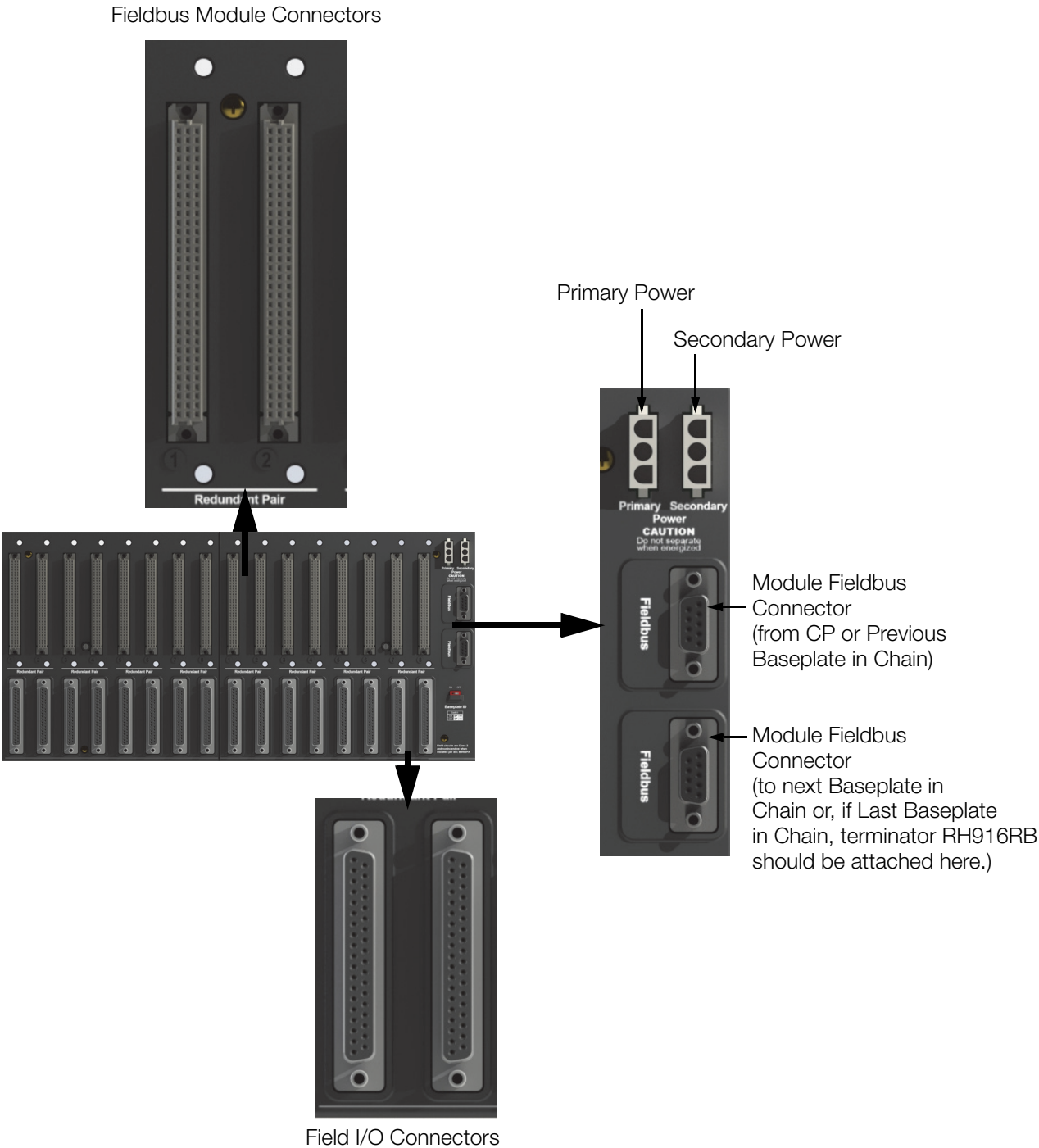
Figure 4. Compact 200 Series Baseplate Connections (Example)
