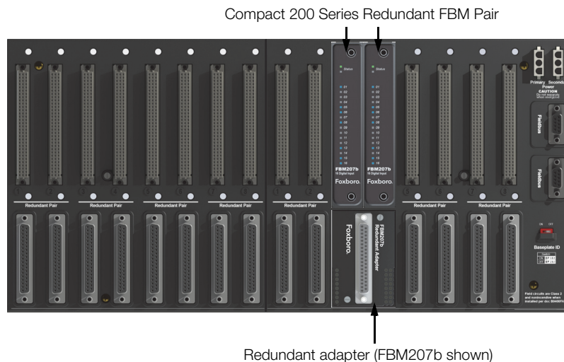
Figure 6. Redundant Adapter
