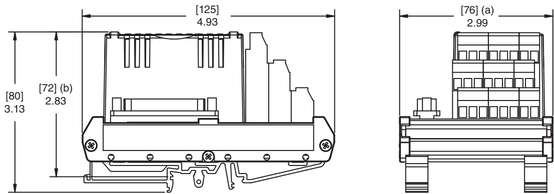
Compression Termination Assembly - RH924JH
