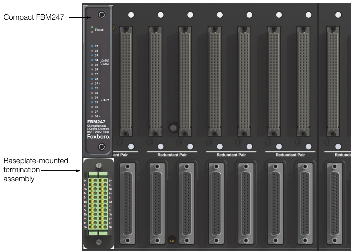
Figure 1. Baseplate-Mounted Termination Assembly
