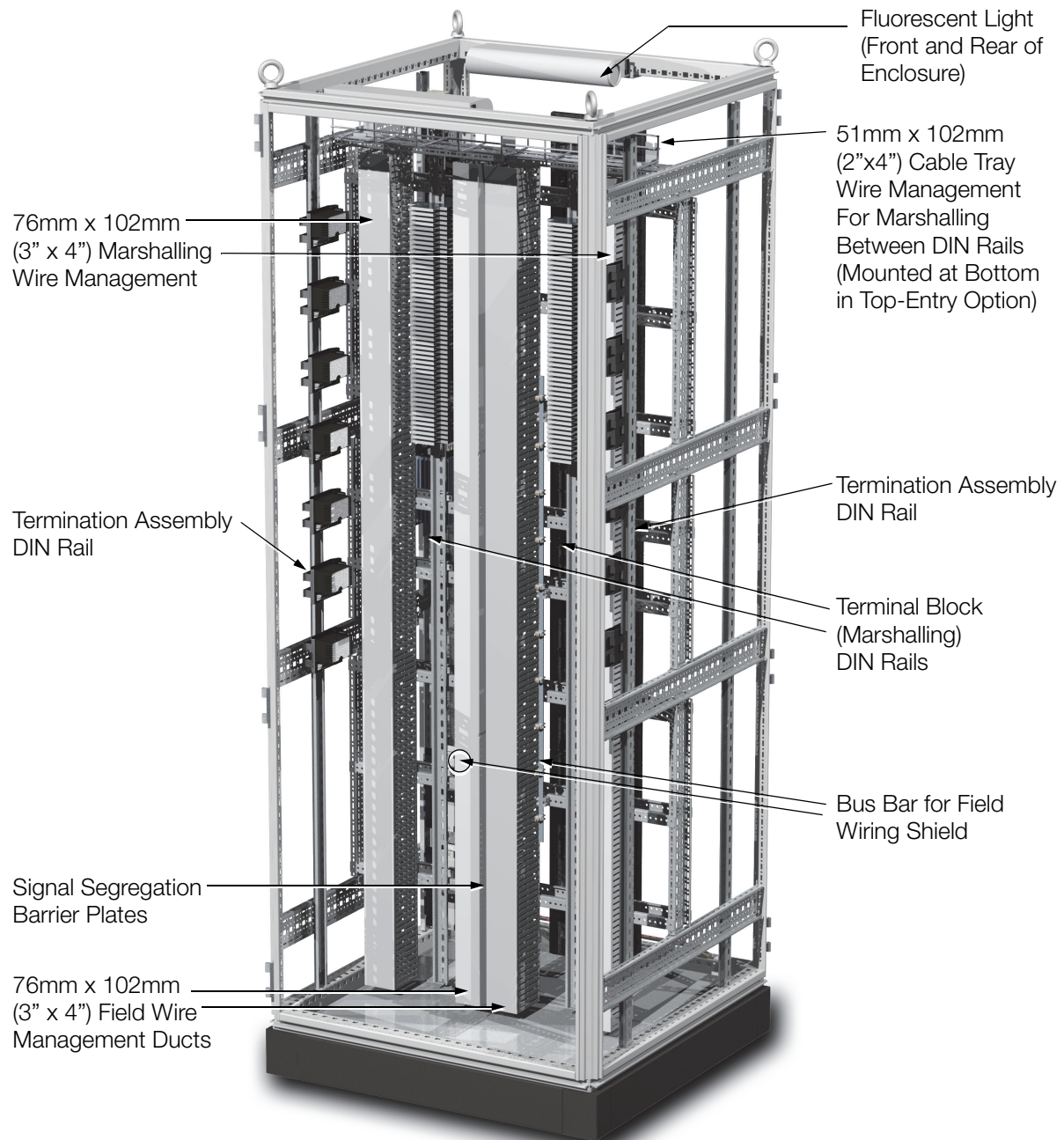
Figure 3. G12 System and Termination Enclosure, Rear View
