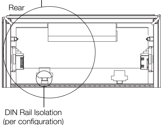
Figure 1. G14 Enclosure Termination and Marshalling Layouts and DIN Rail Identification
