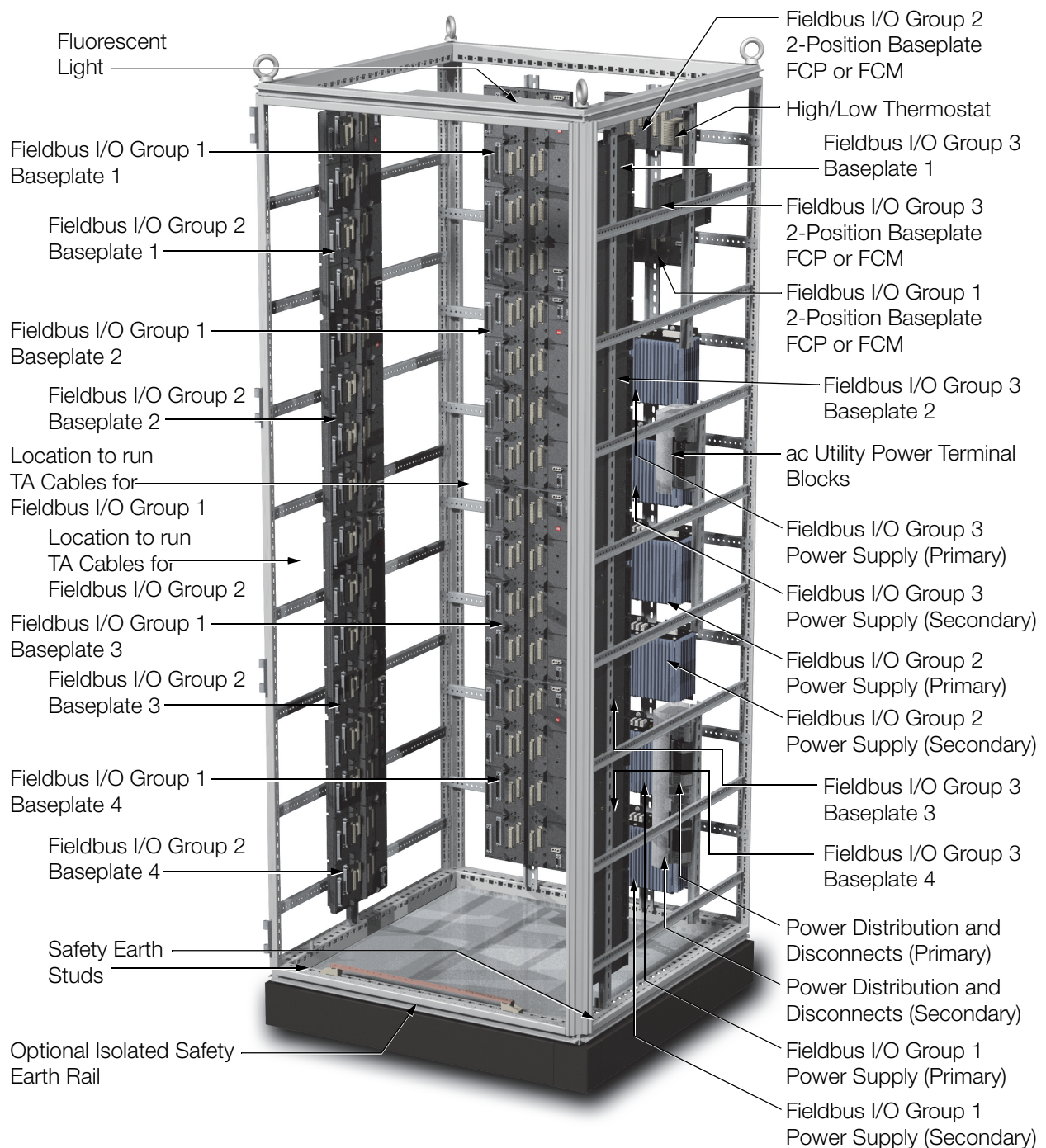
Figure 2. G15 System Enclosure, Front Right View
