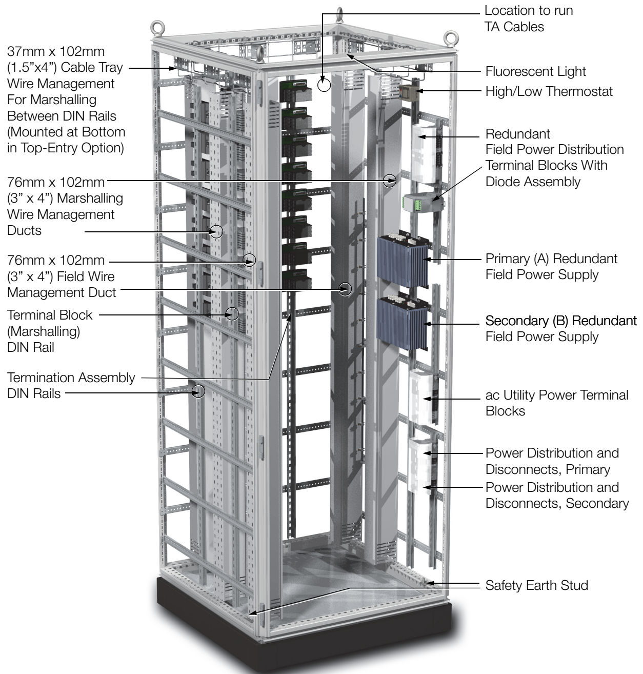
Figure 2. G16 Termination Enclosure with Marshalling Option, Front Left View, Bottom Entry
