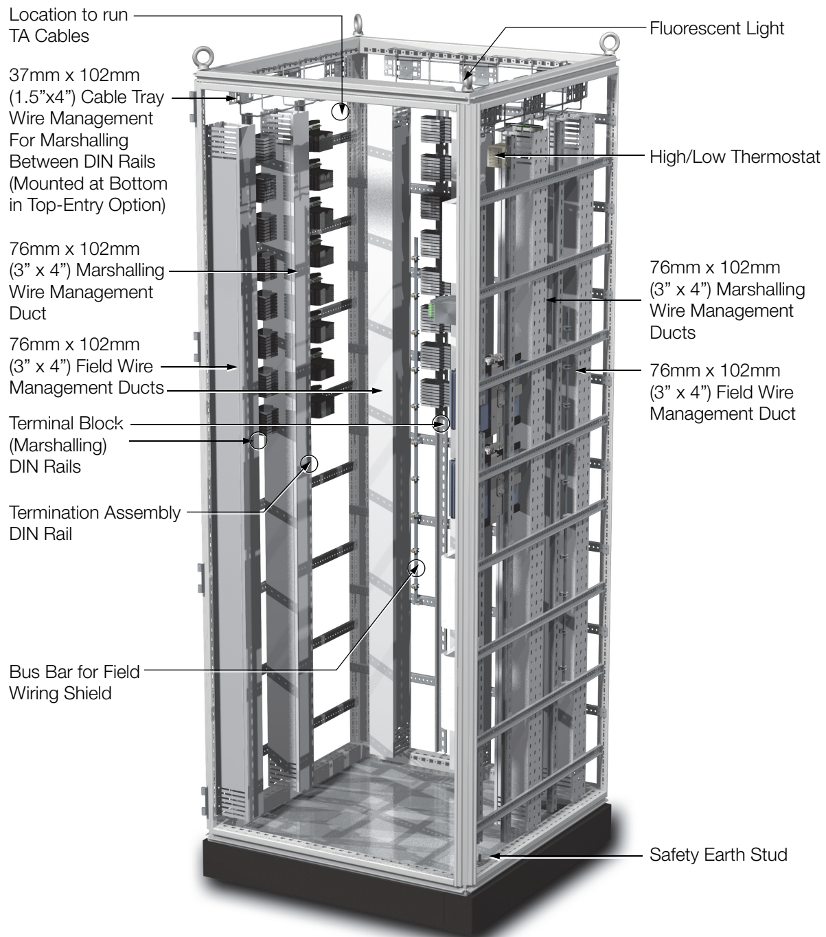
Figure 3. G16 Termination Enclosure with Marshalling Option, Front Right View, Bottom Entry
