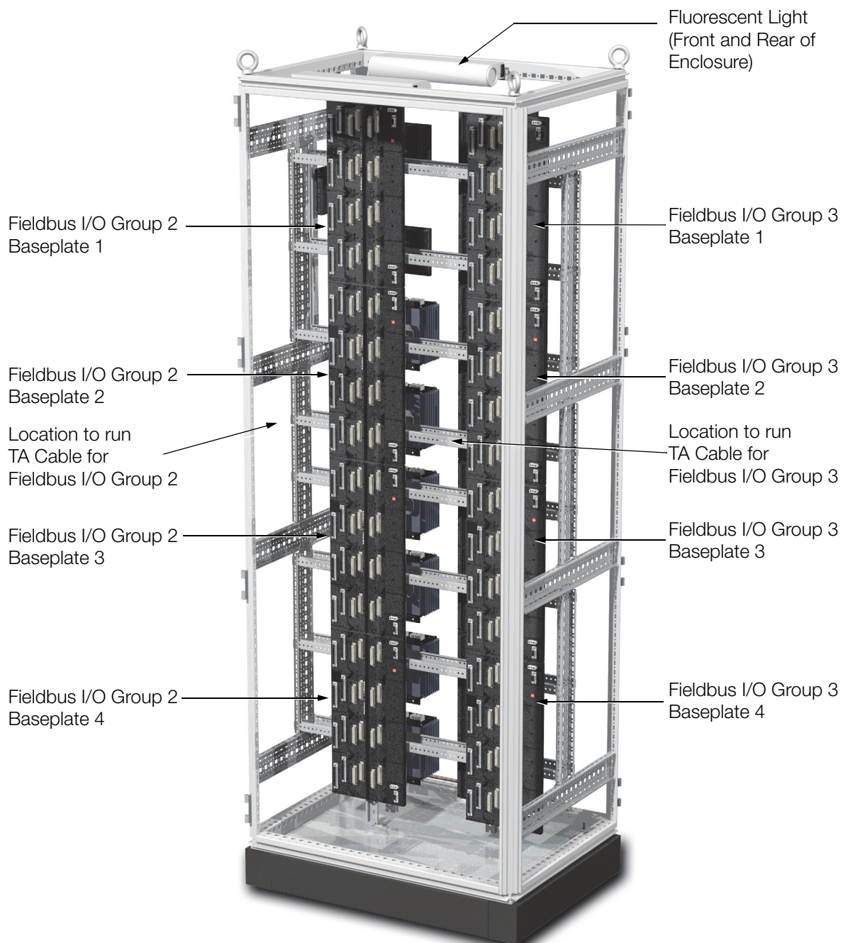
Figure 2. G20 System Enclosure, Rear View
