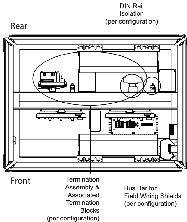
G22 Marshalling Layout
