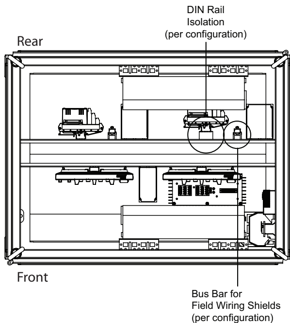
G22 Termination Layout
