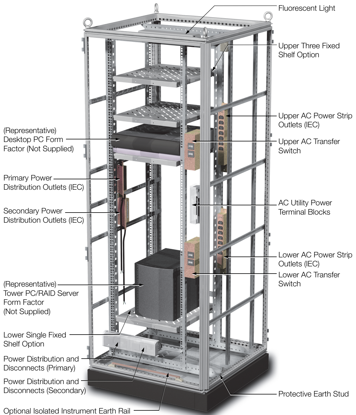
Figure 1. G45 19-Inch Rack Enclosure, Front View with Shelf Options
