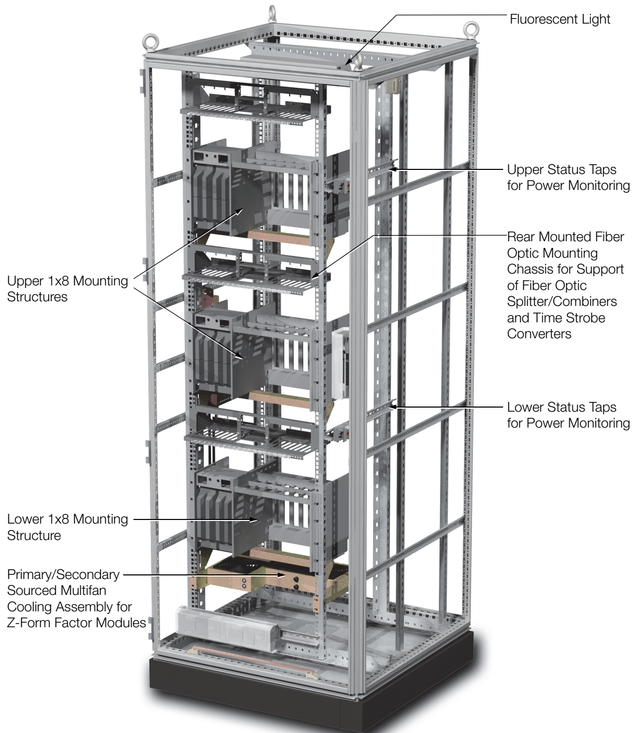
Figure 2. G45 19-Inch Rack Enclosure, Front View With 1x8 Mounting Structure Option
