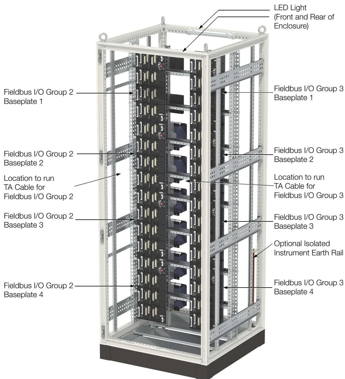
Figure 2. K10 System Enclosure, Rear View
