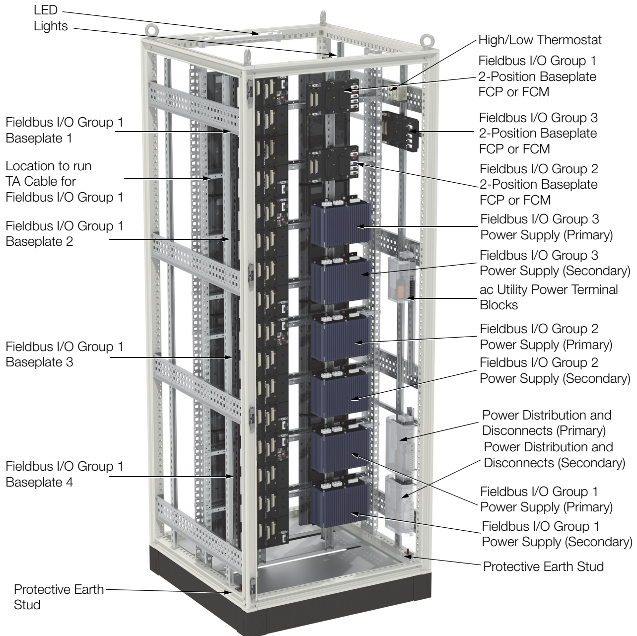
Figure 1. K10 System Enclosure, Front View
