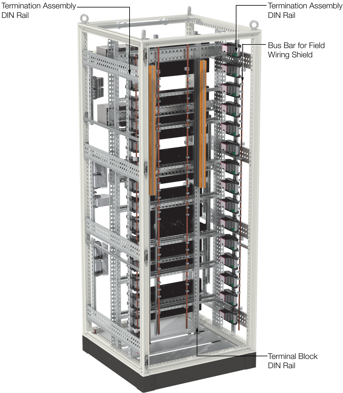
Figure 3. K14 System and Termination Enclosure, Rear View
