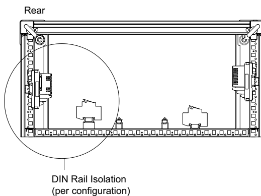
Figure 1. K14 Enclosure Termination and Marshalling Layouts and DIN Rail Identification
