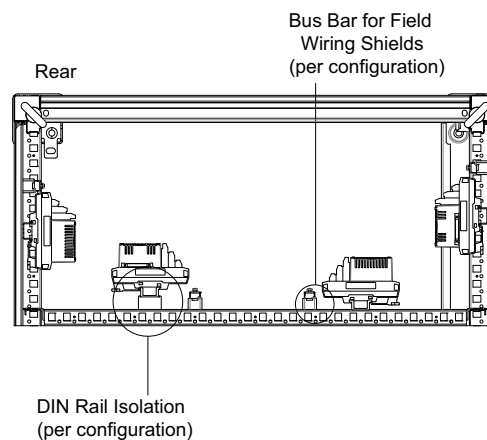
Figure 1. K14 Enclosure Termination and Marshalling Layouts and DIN Rail Identification
