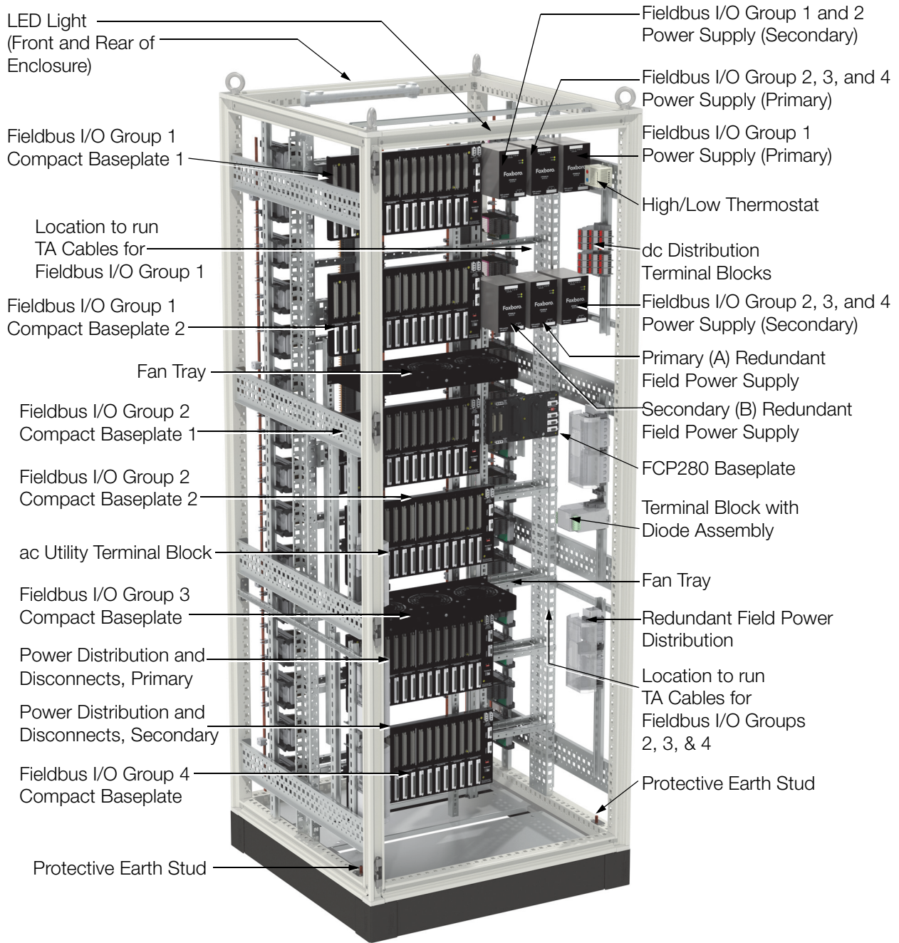
Figure 2. K14 System and Termination Enclosure, Front View
