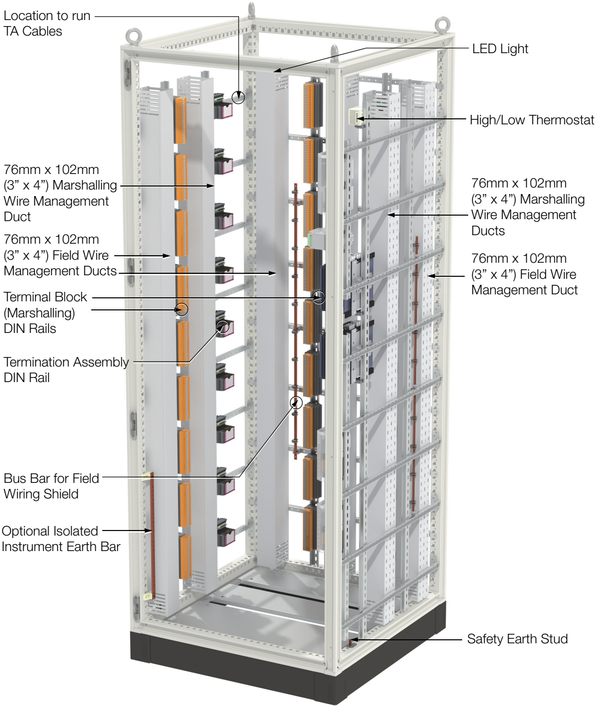
Figure 3. K16 Termination Enclosure with Marshalling Option, Front Right View, Bottom Entry
