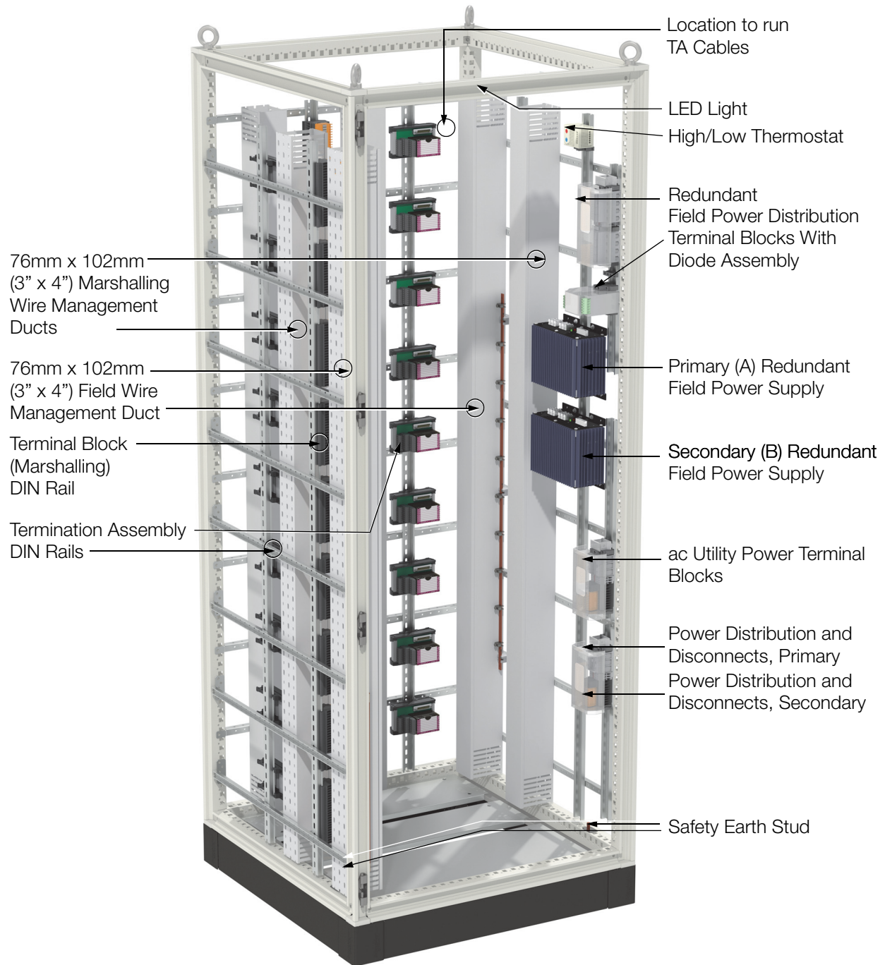
Figure 2. K16 Termination Enclosure with Marshalling Option, Front Left View, Bottom Entry
