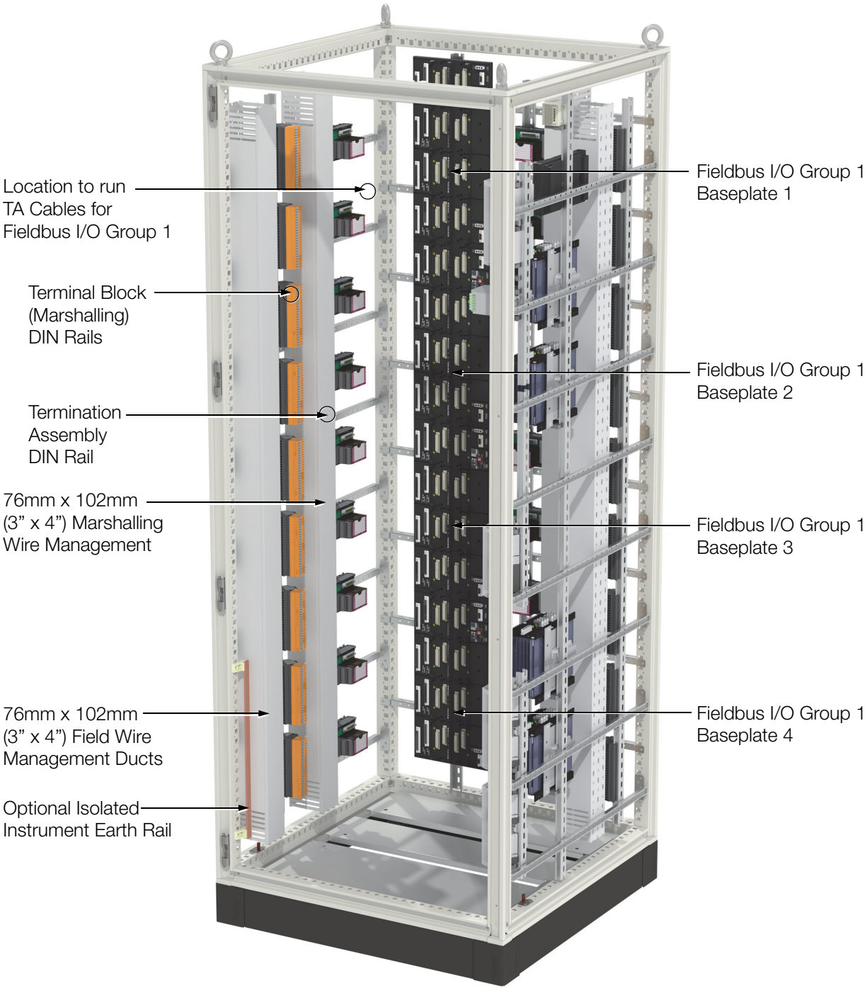
Figure 2. K17 System and Termination Enclosure, Front Right View
