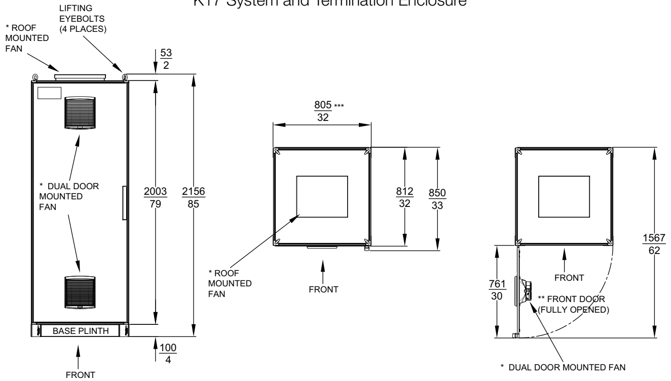
K17 System and Termination Enclosure
