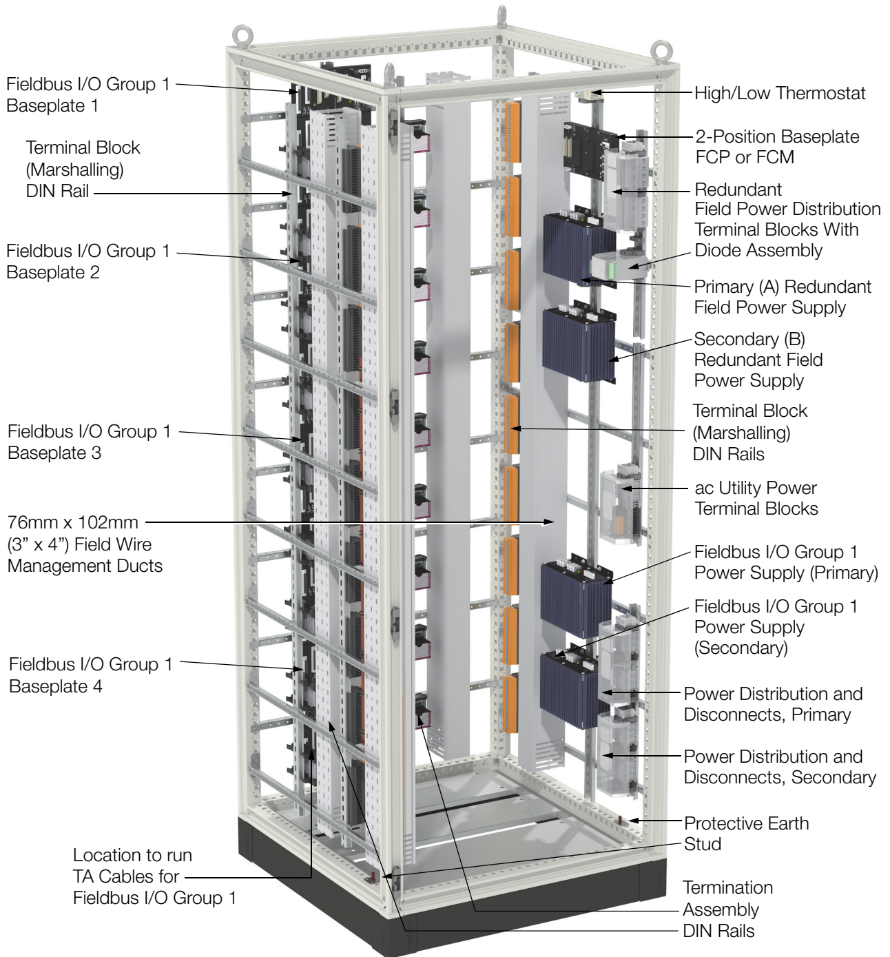
Figure 1. K17 System and Termination Enclosure, Front Left View
