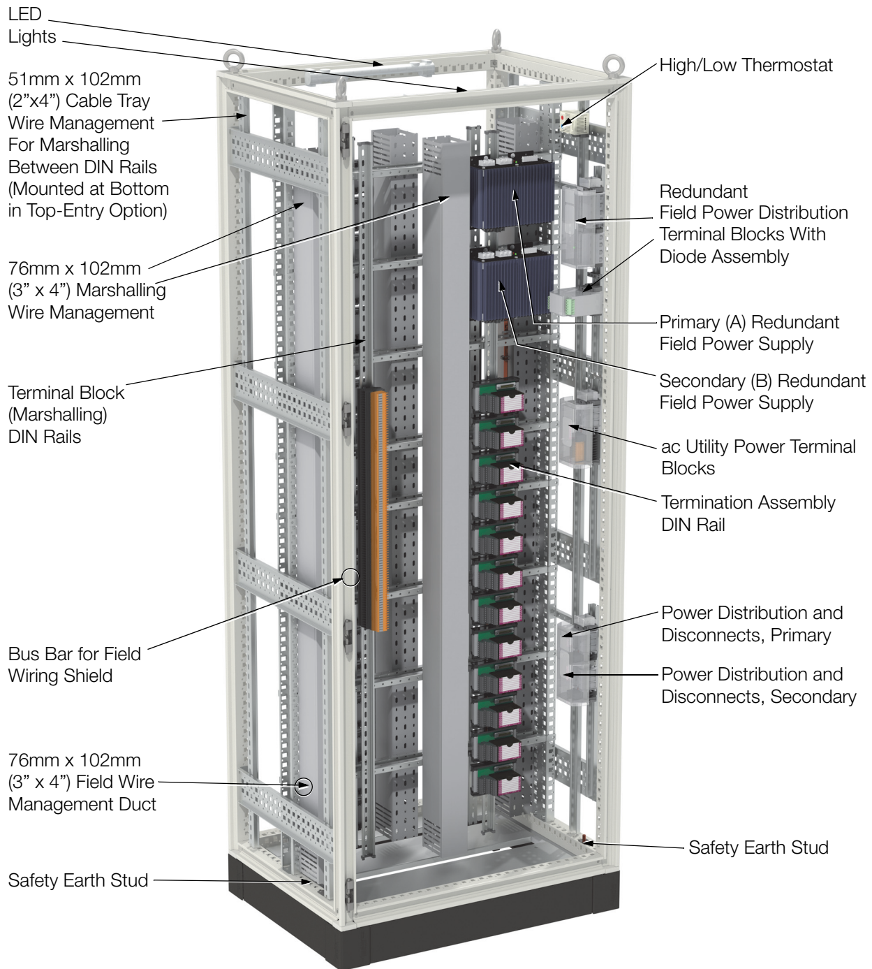
Figure 2. K21 Termination Enclosure with Marshalling Option, Front View, Bottom Entry
