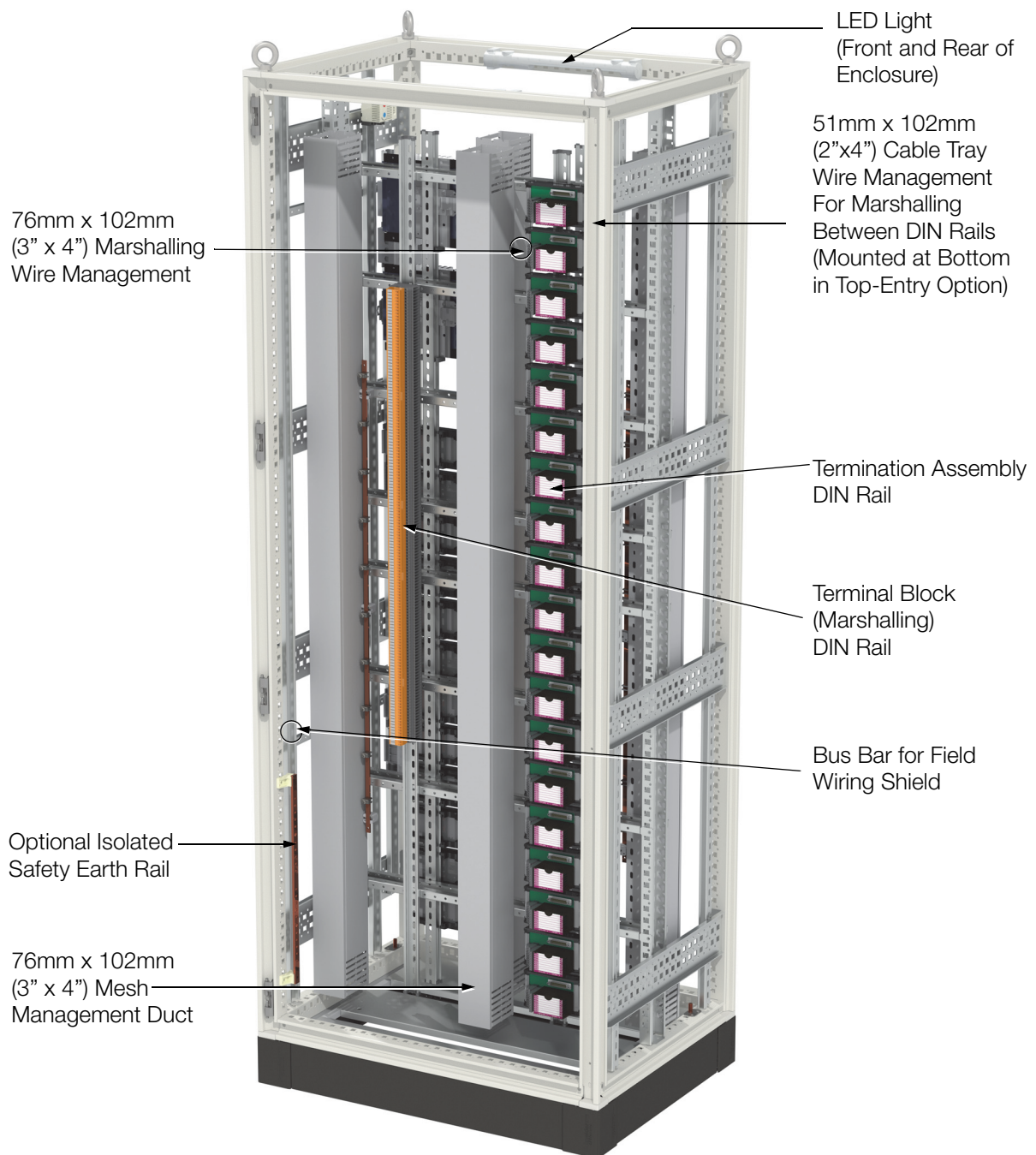
Figure 3. K21 Termination Enclosure with Marshalling Option, Rear View, Bottom Entry
