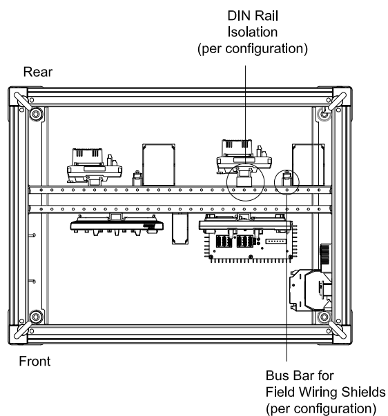
K22 Termination Layout
