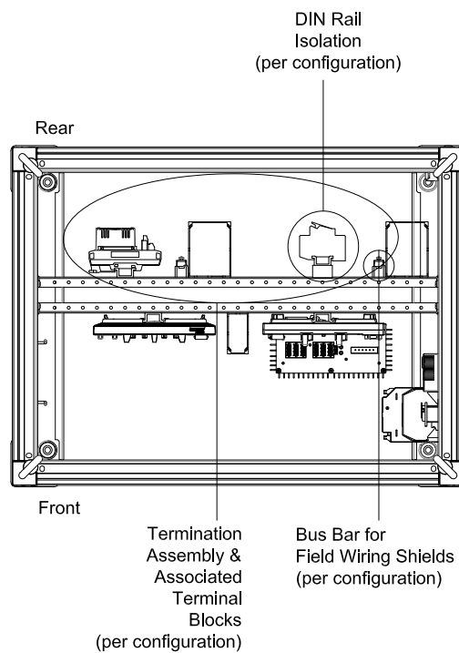
K22 Marshalling Layout
