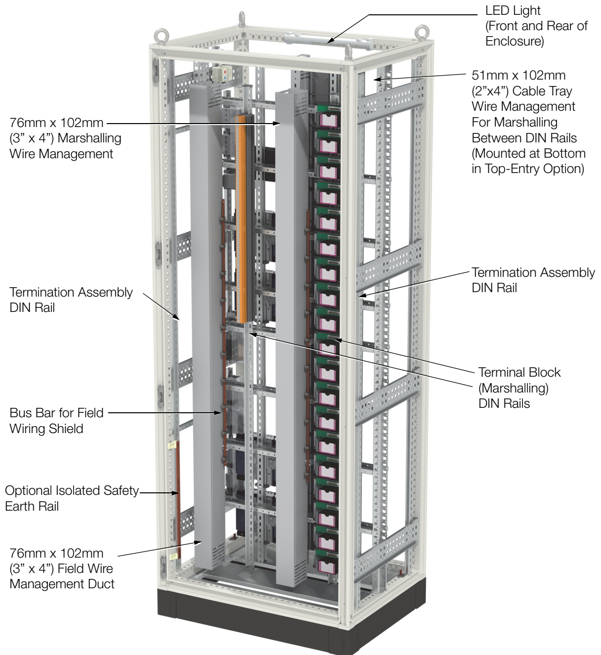
Figure 2. K22 System and Termination Enclosure, Rear View
