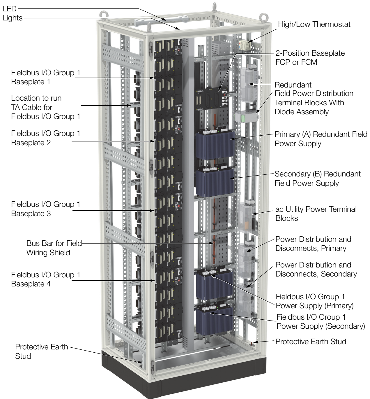
Figure 1. K22 System and Termination Enclosure, Front View
