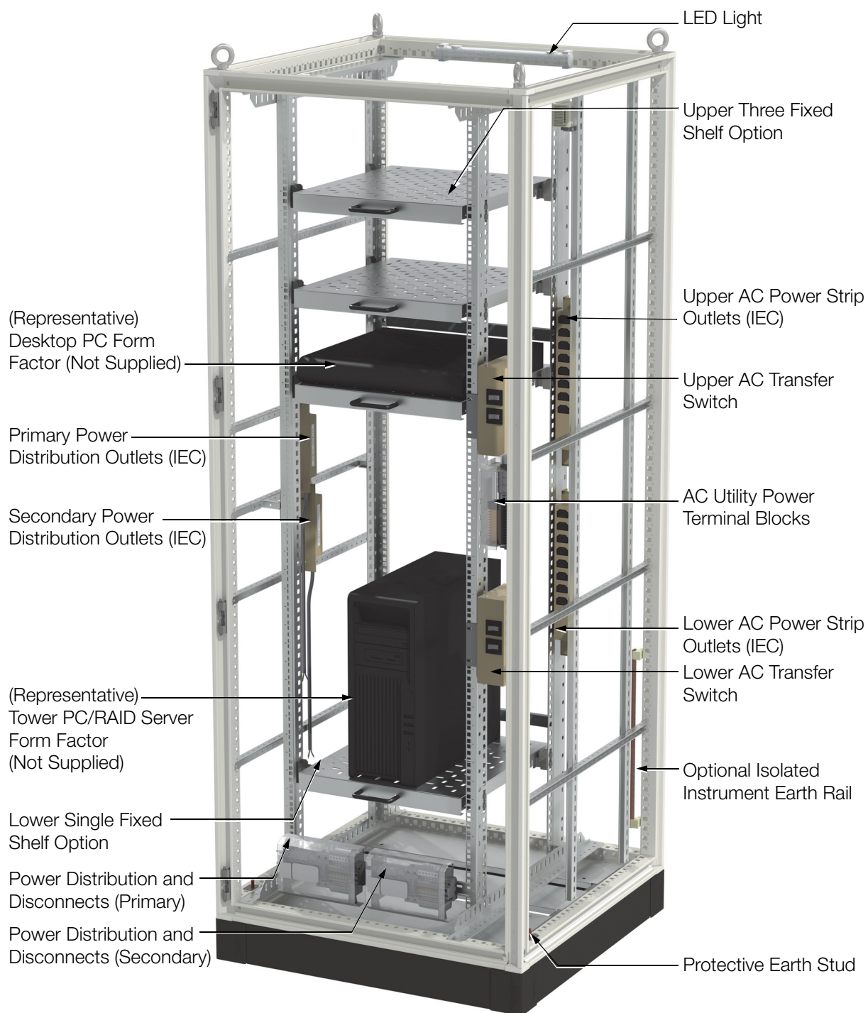
Figure 1. K40 19-Inch Rack Enclosure, Front View with Shelf Options
