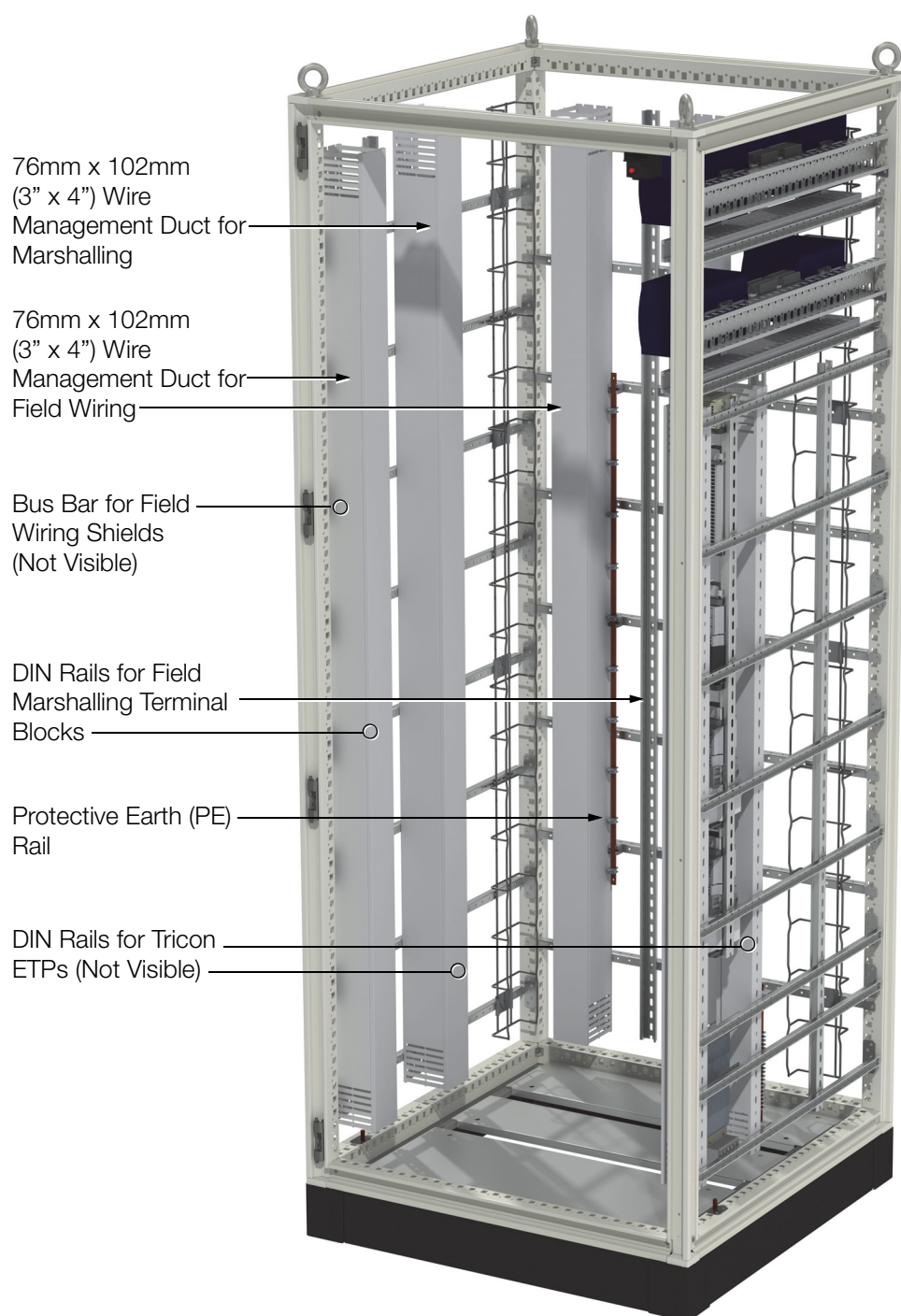
Figure 3. K66 Tricon Termination Enclosure with Marshalling Option, Front Left View, Bottom Entry
