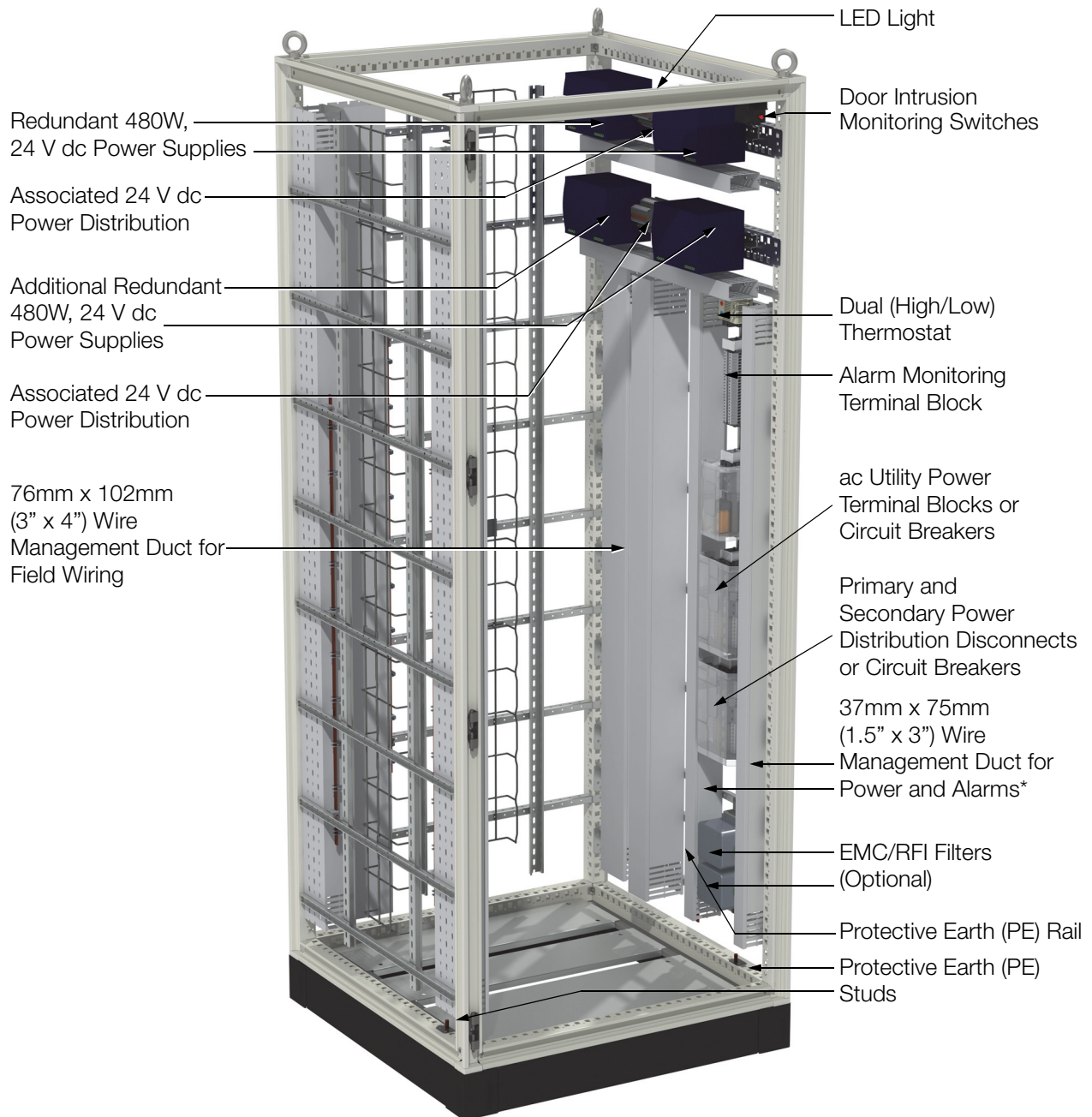
Figure 4. K66 Tricon Termination Enclosure with Termination Option, Front Right View, Bottom Entry
