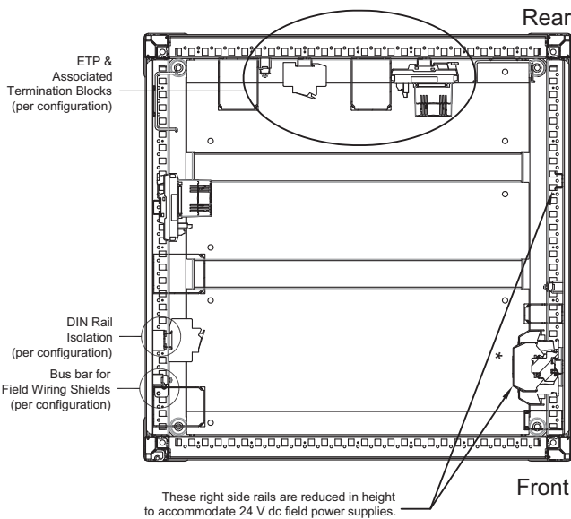
Figure 1. K66 Tricon Termination Enclosure Termination and Marshalling Layouts and DIN Rail Identification
