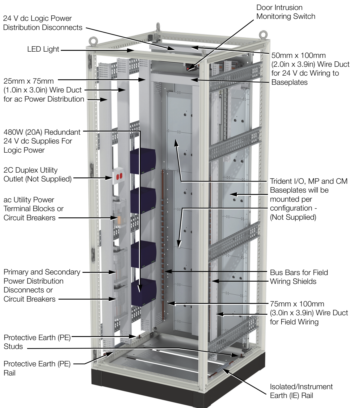
Figure 1. K85 Trident Enclosure, Front Left View
