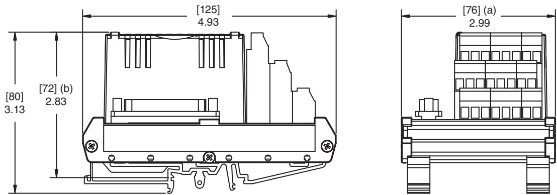
Compression Termination Assembly - RH924JH (supersedes P0924JH)
