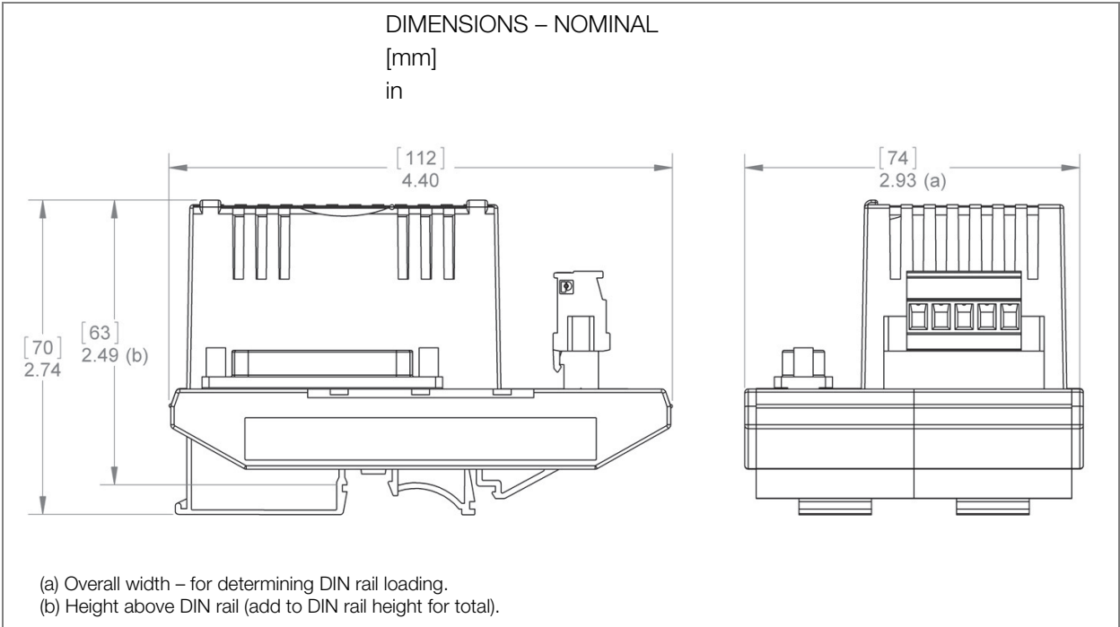
Figure 2. Termination Assembly (RH926TE (supersedes P0926TE))
