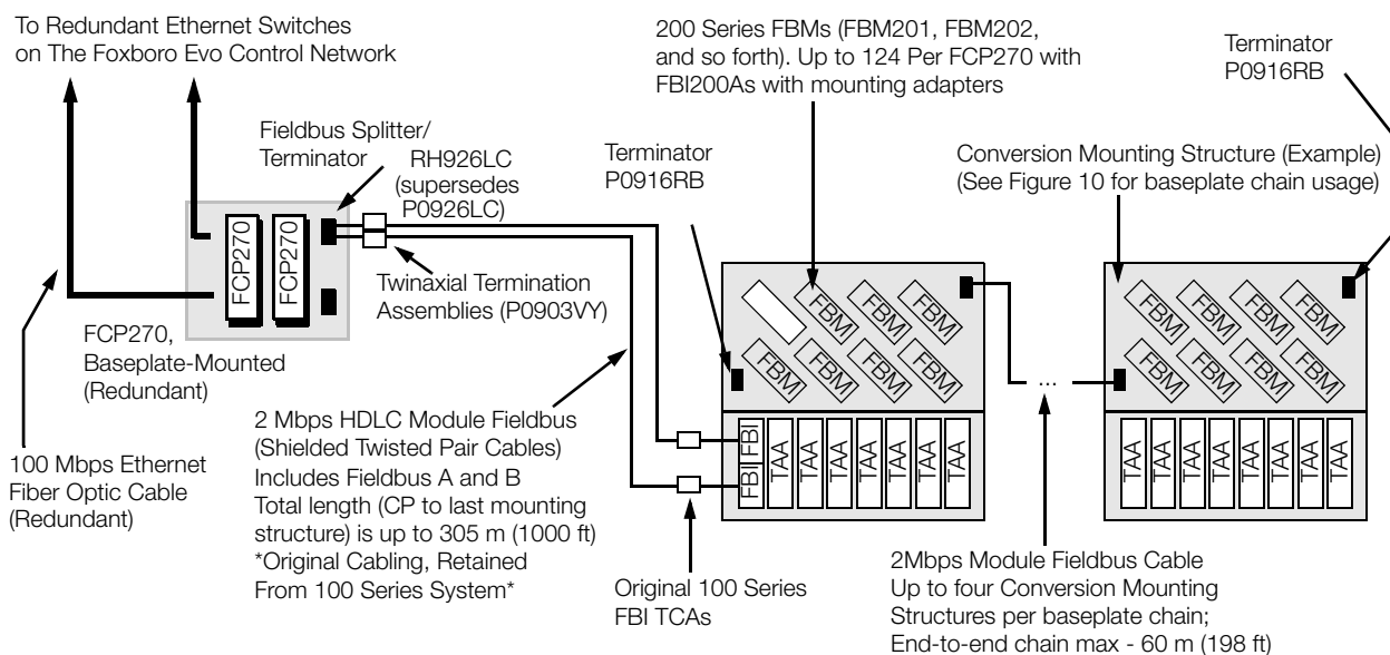
100 SERIES FIELDBUS MODULE UPGRADE SUBSYSTEM WITHOUT FBI200A MODULES
