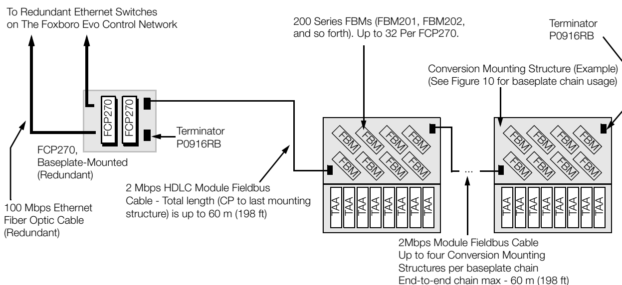
100 SERIES FIELDBUS MODULE UPGRADE SUBSYSTEM WITHOUT FBI200A MODULES
