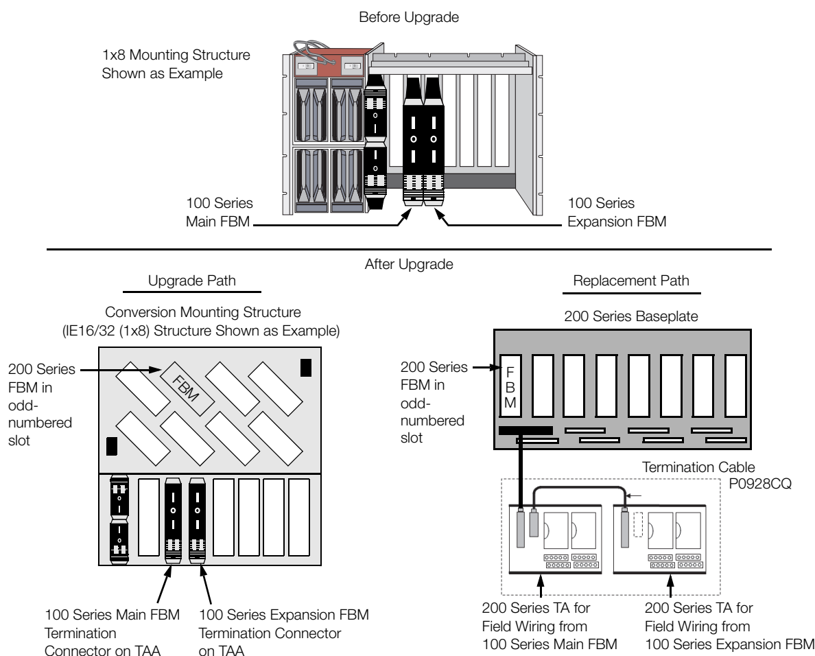
Figure 11. Upgrade for 100 Series Main/Expansion Pair
