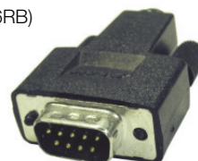
Figure 7. Fieldbus Baseplate Terminator
