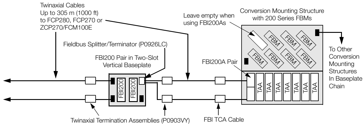
Figure 5. Using FBI200 to Extend 2 Mbps HDLC Module Fieldbus (Conceptual)
