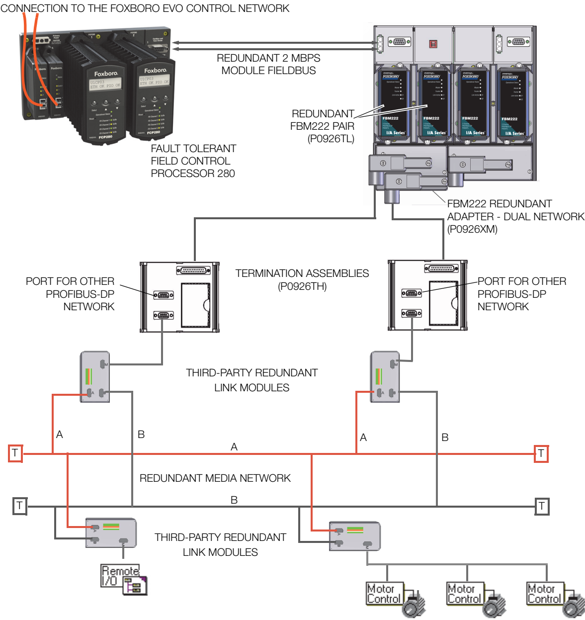
Figure 2. Redundant FBM222s with Redundant Media PROFIBUS-DP Network
