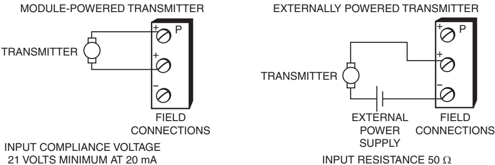
Figure 2. Input Connections
